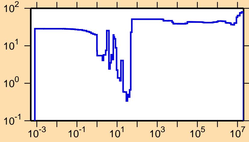
\Delta\sigma/\sigma vs. E for ^{113}\text{Te}(n,\gamma)
