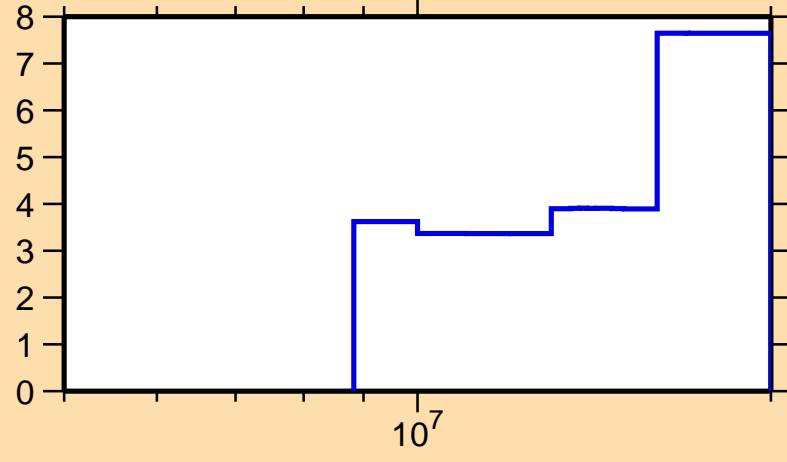
\Delta\sigma/\sigma vs. E for ^{113}\text{Te}(n,\text{el.})
