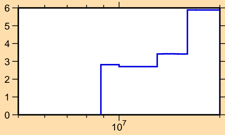
\Delta\sigma/\sigma vs. E for ^{113}\text{Te}(n,\text{tot.})
