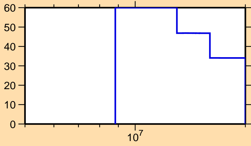
\Delta\sigma/\sigma vs. E for ^{113}\text{Te}(n,2n)
