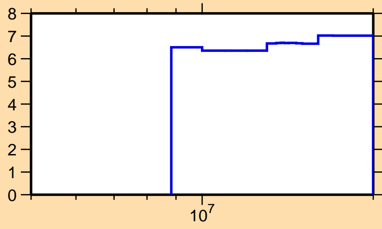
\Delta\sigma/\sigma vs. E for ^{113}\text{Te}(n,\text{nonel.})
