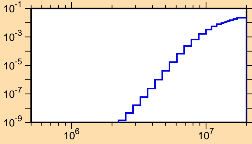
\sigma vs. E for ^{113}\text{Te}(n,p\alpha)
