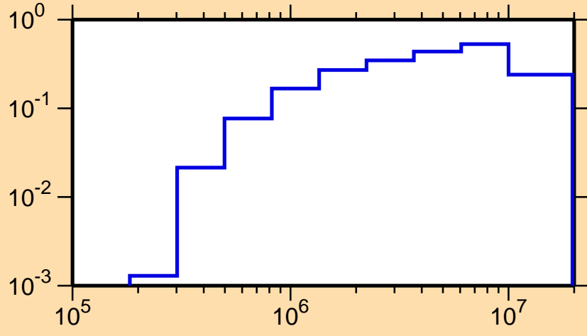
\sigma vs. E for ^{113}\text{Te}(n,n\text{cont.})
