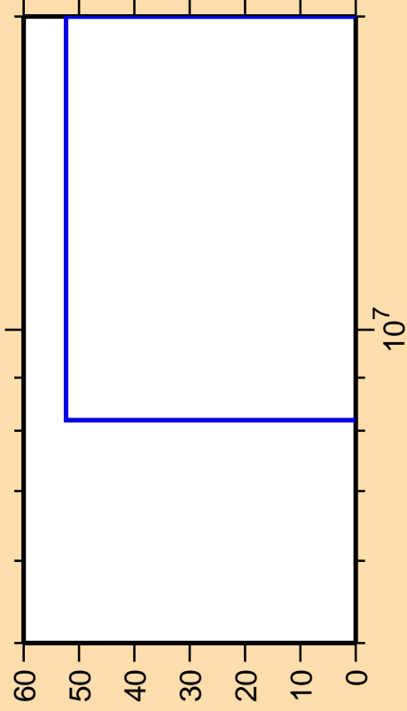
\Delta\sigma/\sigma vs. E for ^{113}\text{Te}(n,2n\alpha)
