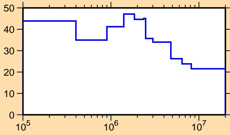
\Delta\sigma/\sigma vs. E for ^{113}\text{Te}(n,n_1)
