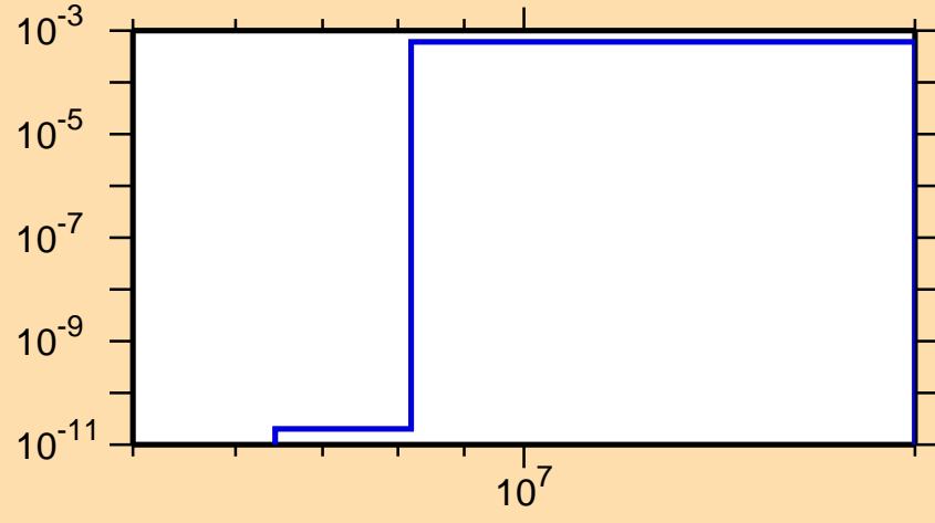
\sigma vs. E for ^{113}\text{Te}(n,t)
