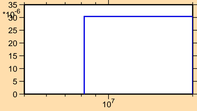
\sigma vs. E for ^{113}\text{Te}(n,2np)
