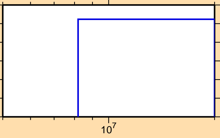
\sigma vs. E for ^{113}\text{Te}(n,pd)
