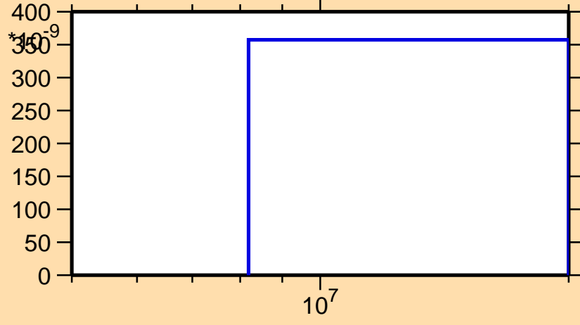
\sigma vs. E for ^{113}\text{Te}(\text{mt } 45)
