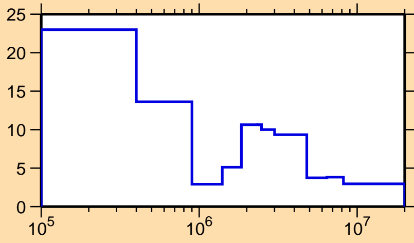
\Delta\sigma/\sigma vs. E for ^{113}\text{Te}(n,\text{tot.})
