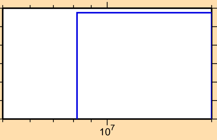
\sigma vs. E for ^{113}\text{Te}(n,2n\alpha)
