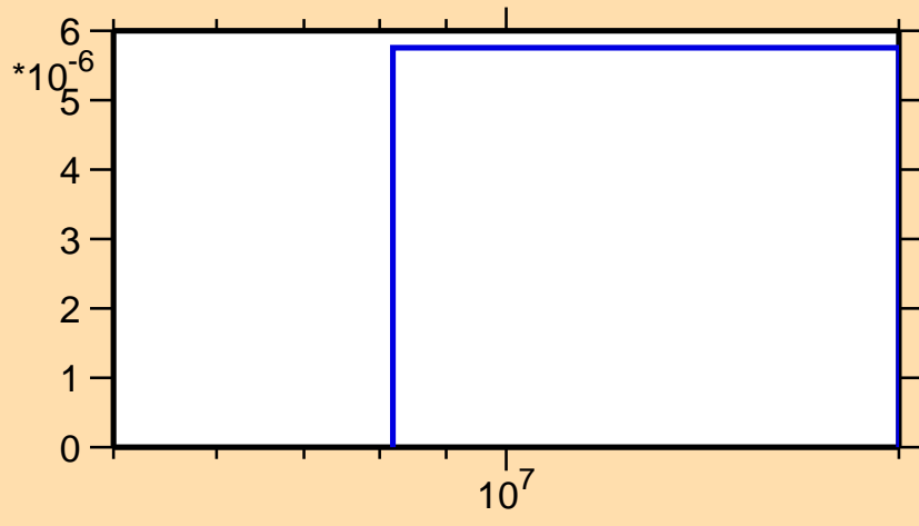
\sigma vs. E for ^{113}\text{Te}(n,2n\alpha)
