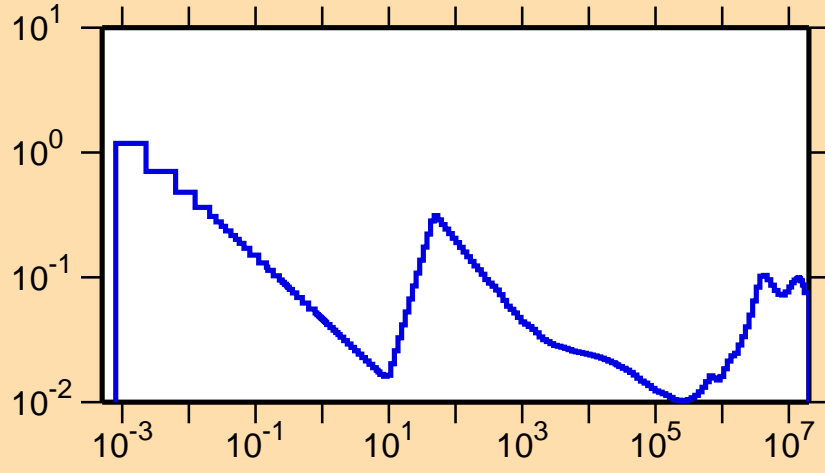
\sigma vs. E for ^{114}\text{Te}(n,\alpha)
