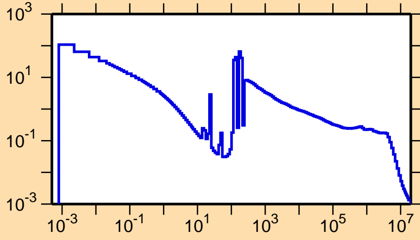
\sigma vs. E for ^{114}\text{Te}(n,\gamma)
