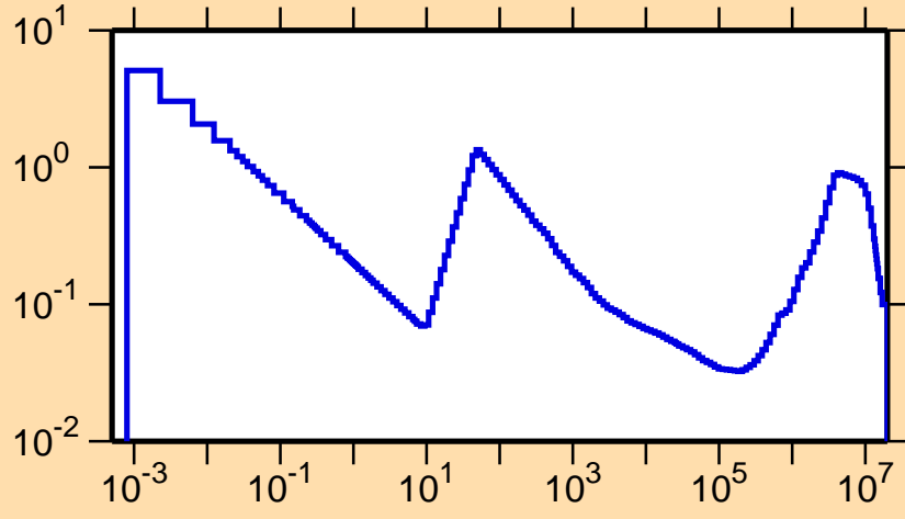
\sigma vs. E for ^{114}\text{Te}(n,p)
