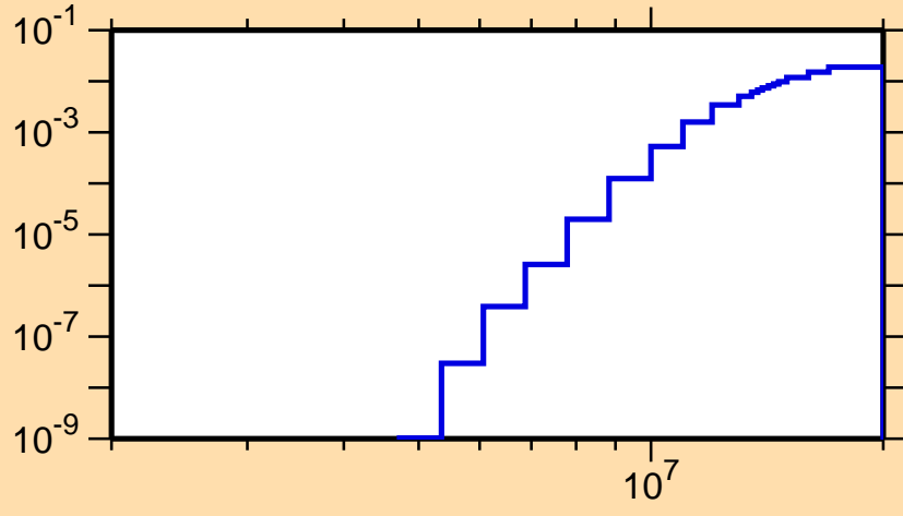
\sigma vs. E for ^{114}\text{Te}(n,d)
