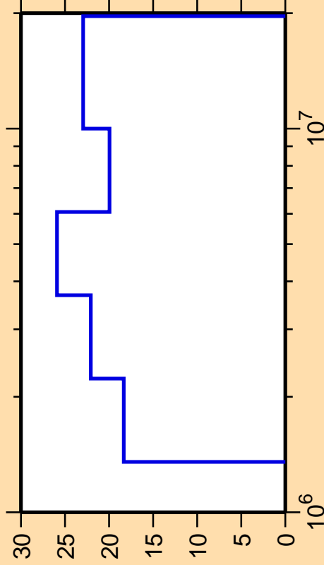
\Delta\sigma/\sigma vs. E for ^{114}\text{Te}(n,n_4)
