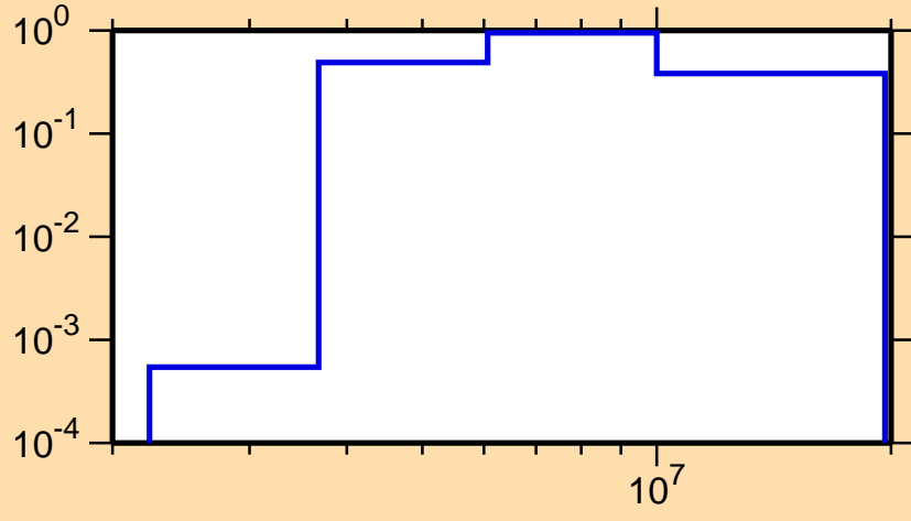
\sigma vs. E for ^{114}\text{Te}(n,n\text{cont.})
