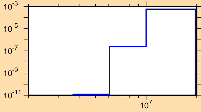
\sigma vs. E for ^{114}\text{Te}(n,p\alpha)
