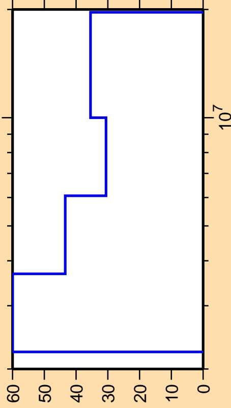
\Delta\sigma/\sigma vs. E for ^{114}\text{Te}(n,n\text{cont.})
