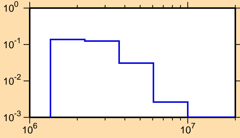
\sigma vs. E for ^{114}\text{Te}(n,n_4)
