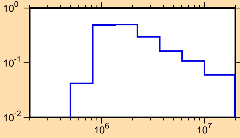
\sigma vs. E for ^{114}\text{Te}(n,n_1)
