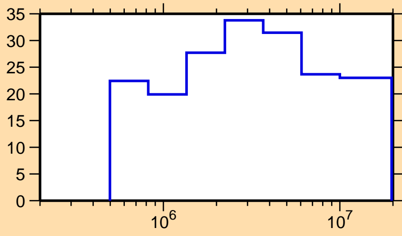
\Delta\sigma/\sigma vs. E for ^{114}\text{Te}(n,n_1)
