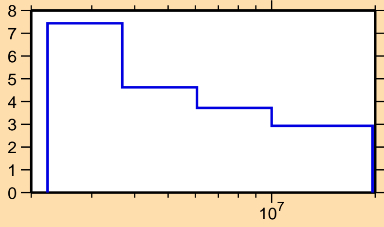
\Delta\sigma/\sigma vs. E for ^{114}\text{Te}(n,\text{nonel.})
