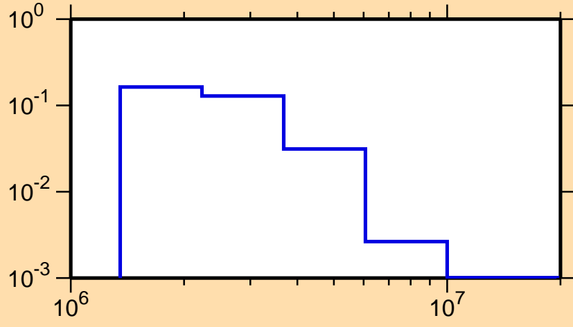
\sigma vs. E for ^{114}\text{Te}(n,n_2)
