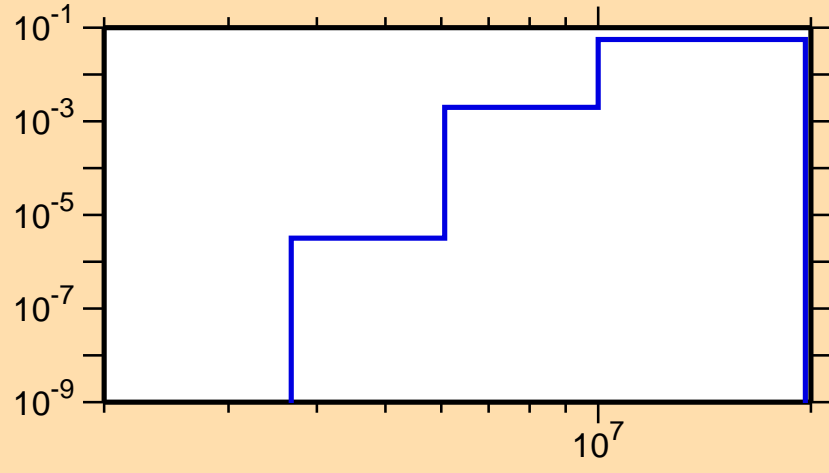
\sigma vs. E for ^{114}\text{Te}(n,n\alpha)
