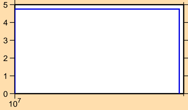
\Delta\sigma/\sigma vs. E for ^{114}\text{Te}(n,\text{el.})
