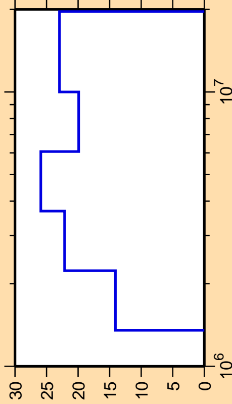
\Delta\sigma/\sigma vs. E for ^{114}\text{Te}(n,n_2)
