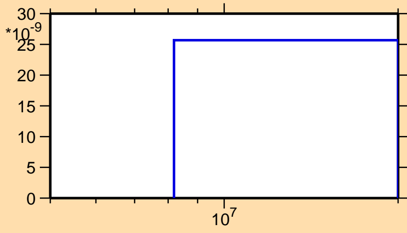
\sigma vs. E for ^{114}\text{Te}(\text{mt } 45)
