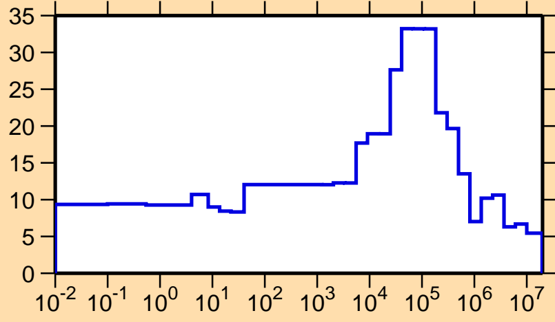
\Delta\sigma/\sigma vs. E for ^{115}\text{Te}(n,el.)
