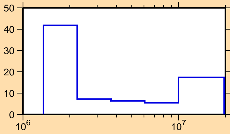
\Delta\sigma/\sigma vs. E for ^{117}\text{Te}(n,n\text{cont.})
