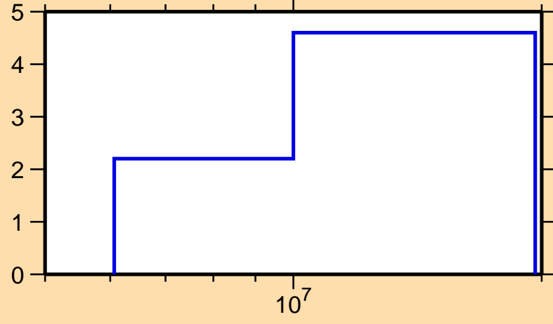
\Delta\sigma/\sigma vs. E for ^{117}\text{Te}(n,\text{el.})
