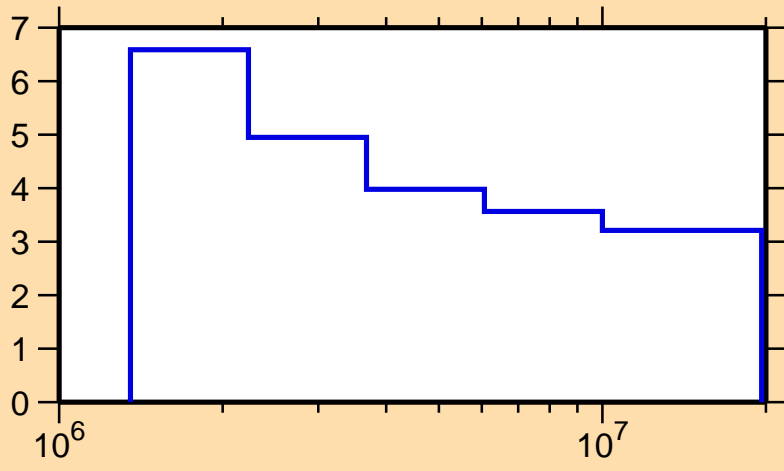
\Delta\sigma/\sigma vs. E for ^{117}\text{Te}(n,n\text{onel.})
