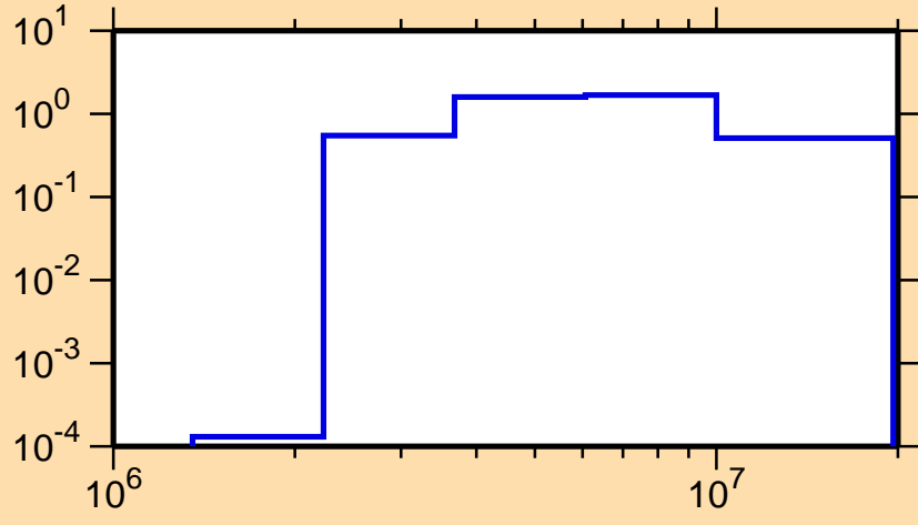
\sigma vs. E for ^{117}\text{Te}(n,n\text{cont.})
