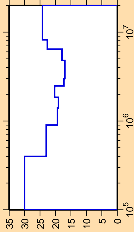
\Delta\sigma/\sigma vs. E for ^{117}\text{Te}(n,n_3)
