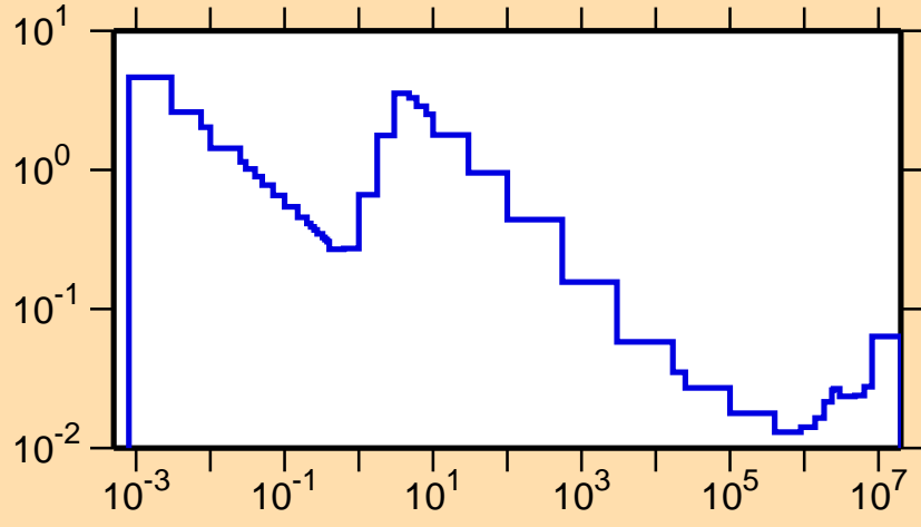
\sigma vs. E for ^{117}\text{Te}(n,\alpha)
