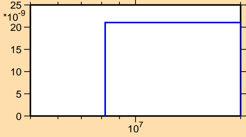
\sigma vs. E for ^{117}\text{Te}(n,3n)
