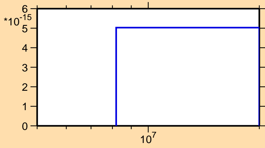
\sigma vs. E for ^{118}\text{Te}(\text{mt } 34)
