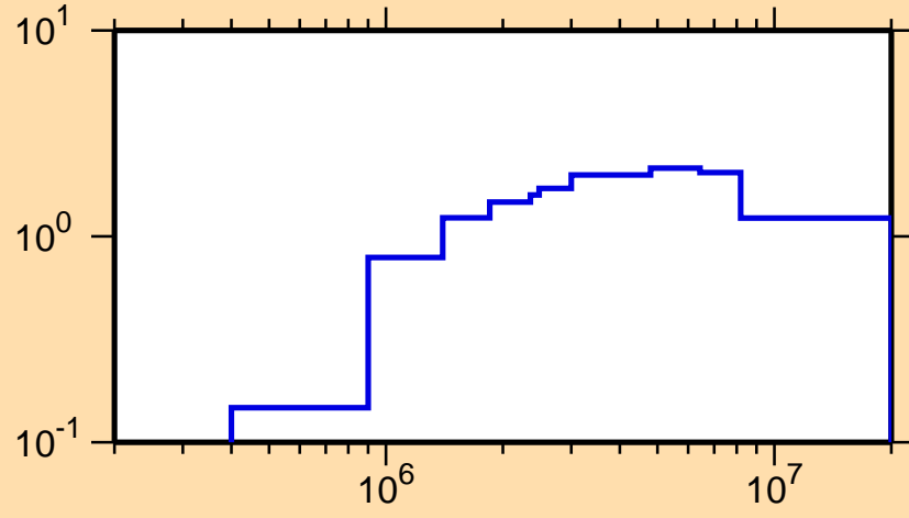
\sigma vs. E for ^{118}\text{Te}(n,\text{inel.})
