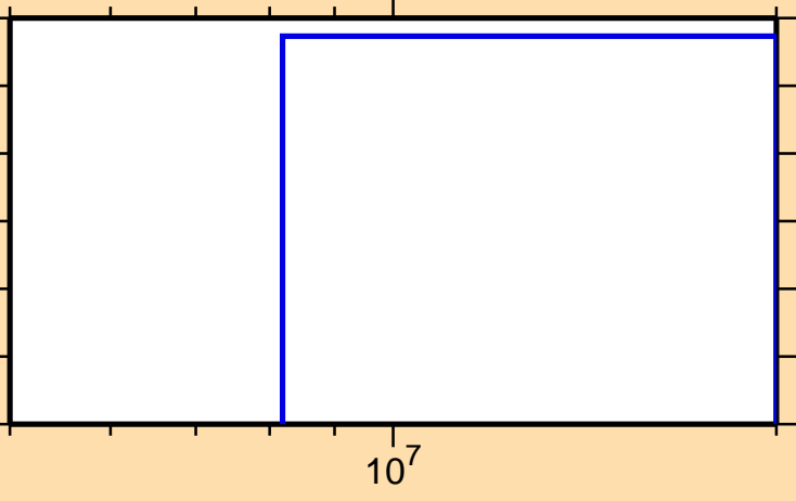
\sigma vs. E for ^{118}\text{Te}(n,pd)
