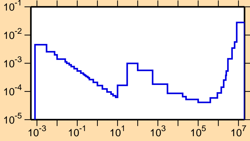
\sigma vs. E for ^{118}\text{Te}(n,\alpha)
