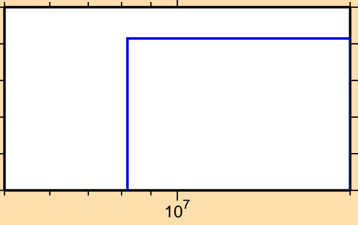
\sigma vs. E for ^{118}\text{Te}(n,\text{He3})
