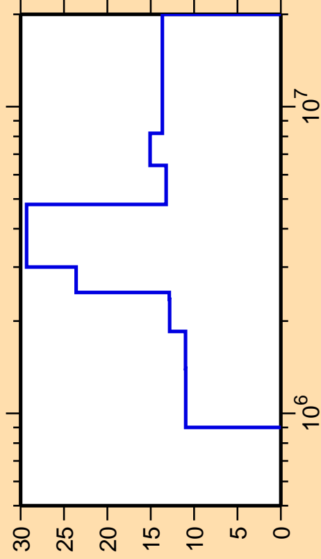
\Delta\sigma/\sigma vs. E for ^{118}\text{Te}(n,n_4)
