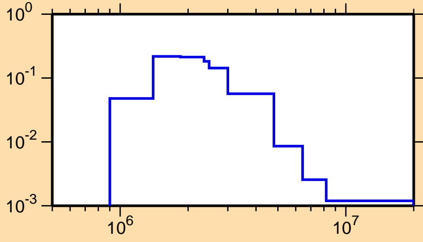
\sigma vs. E for ^{118}\text{Te}(n,n_4)
