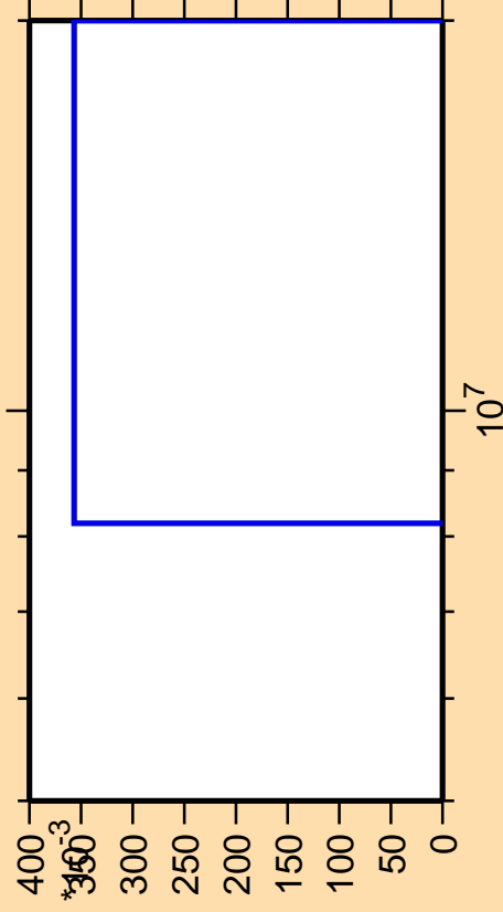
\Delta\sigma/\sigma vs. E for ^{118}\text{Te}(\text{mt } 45)
