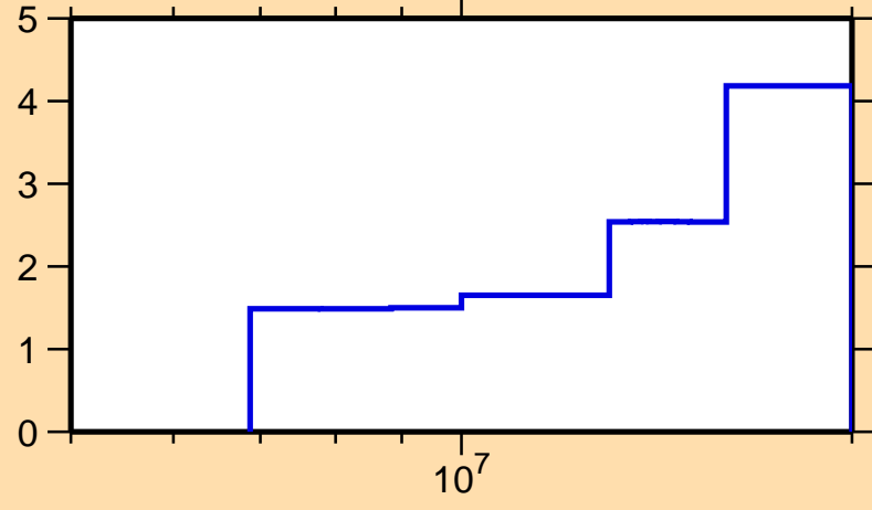
\Delta\sigma/\sigma vs. E for ^{119}\text{Te}(n,tot.)
