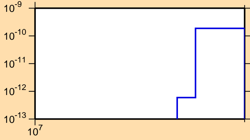
\sigma vs. E for ^{119}\text{Te} (mt 34)
