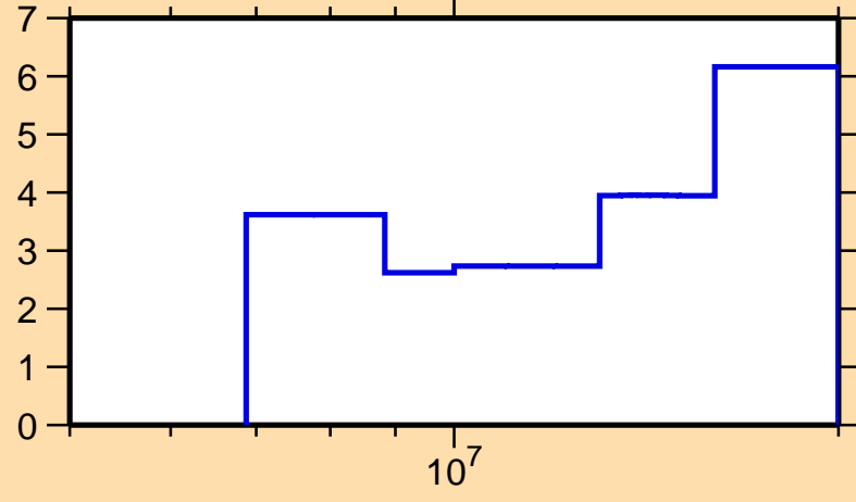
\Delta\sigma/\sigma vs. E for ^{119}\text{Te}(n,\text{el.})
