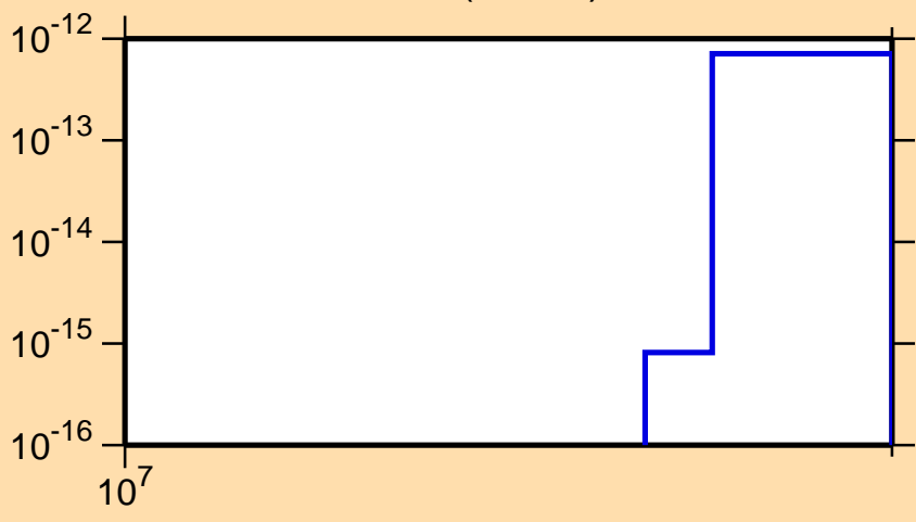
\sigma vs. E for ^{119}\text{Te}(\text{mt } 45)
