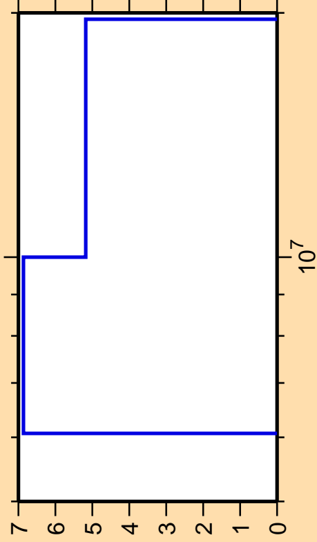
\Delta\sigma/\sigma vs. E for ^{119}\text{Te}(n,2n)
