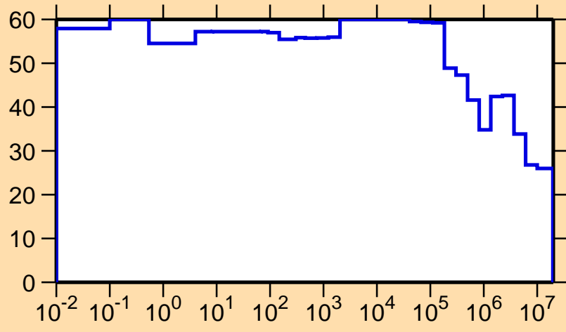
\Delta\sigma/\sigma vs. E for ^{119}\text{Te}(n,p)
