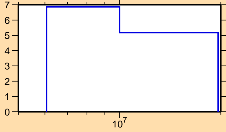
\Delta\sigma/\sigma vs. E for ^{119}\text{Te}(n,2n)
