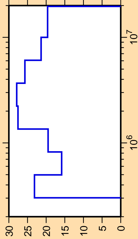
\Delta\sigma/\sigma vs. E for ^{119}\text{Te}(n,n_4)
