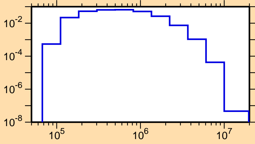
\sigma vs. E for ^{119}\text{Te}(n,n_4)
