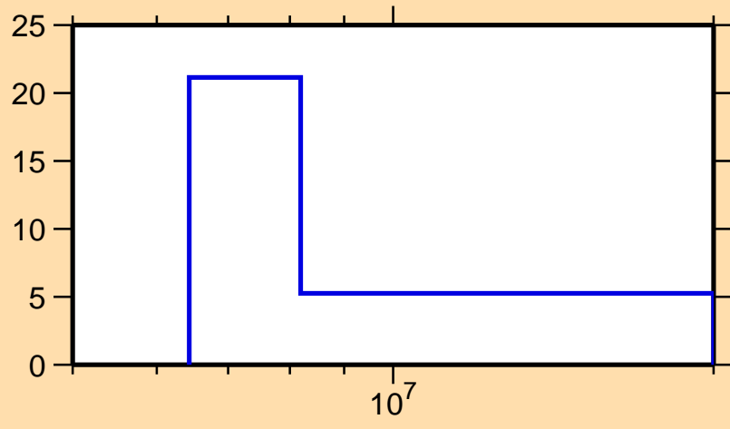
\Delta\sigma/\sigma vs. E for ^{119}\text{Te}(n,2n)
