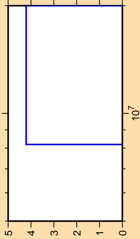
\Delta\sigma/\sigma vs. E for ^{119}\text{Te} (mt 34)
