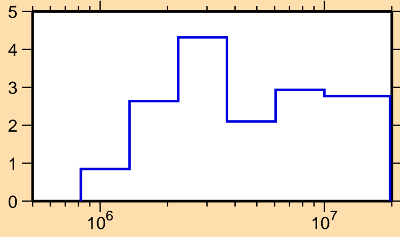
\Delta\sigma/\sigma vs. E for ^{120}\text{Te}(n,el.)
