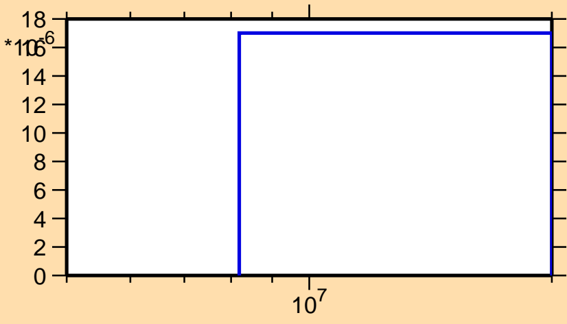
\sigma vs. E for ^{120}\text{Te}(n,t)
