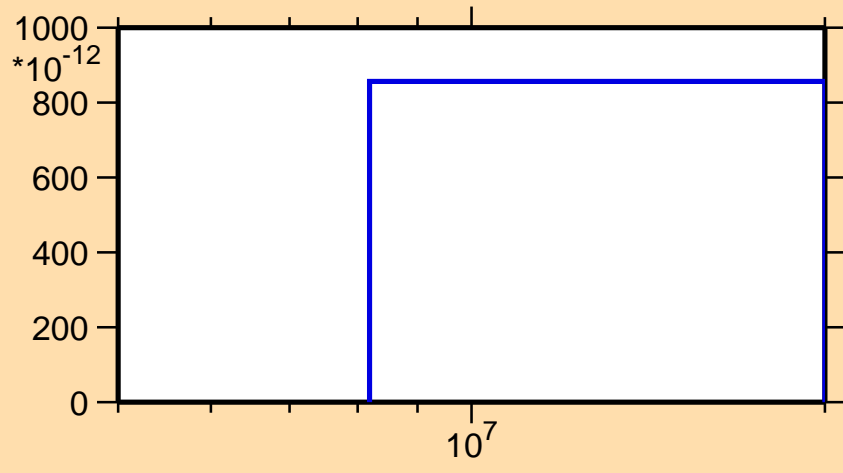
\sigma vs. E for ^{120}\text{Te}(n,nd)
