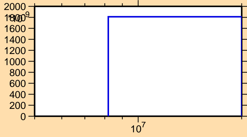
\sigma vs. E for ^{120}\text{Te}(n,3n)
