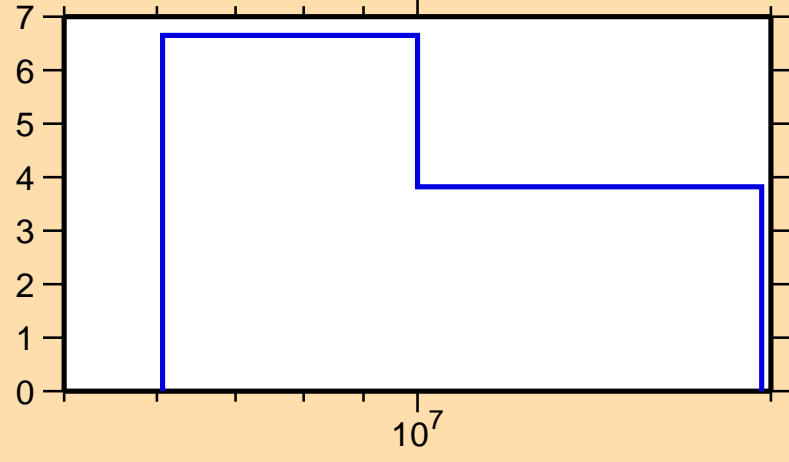
\Delta\sigma/\sigma vs. E for ^{121}\text{Te}(n,2n)
