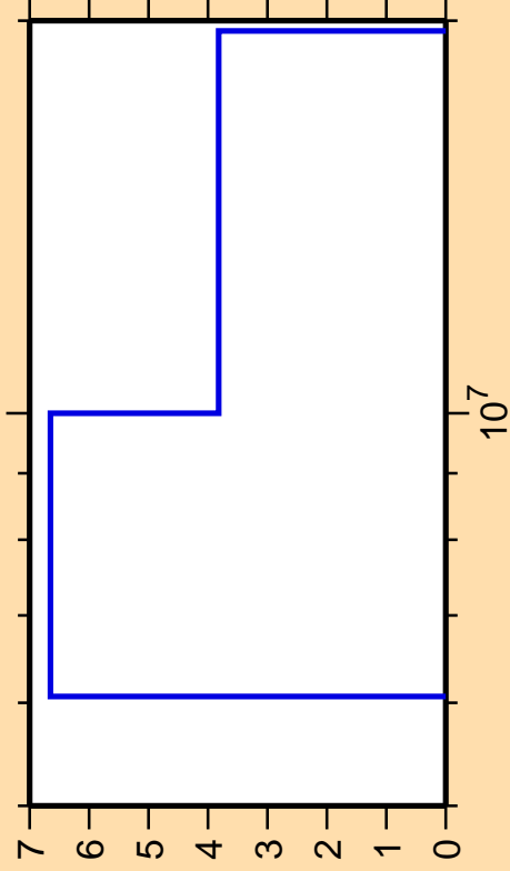
\Delta\sigma/\sigma vs. E for ^{121}\text{Te}(n,2n)
