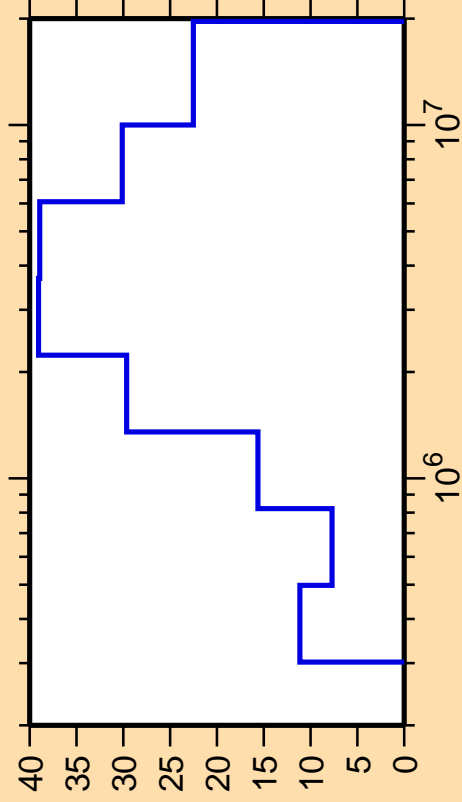
\Delta\sigma/\sigma vs. E for ^{121}\text{Te}(n,n_4)
