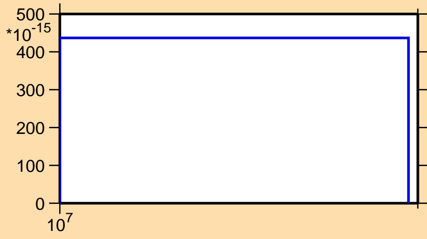
\sigma vs. E for ^{121}\text{Te}(n,pd)
