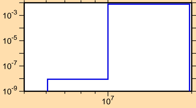
\sigma vs. E for ^{121}\text{Te}(n,np)
