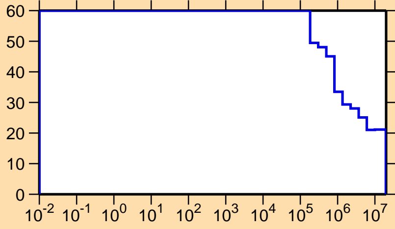
\Delta\sigma/\sigma vs. E for ^{121}\text{Te}(n,p)
