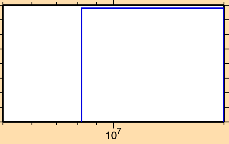
\sigma vs. E for ^{121}\text{Te}(n,p\alpha)
