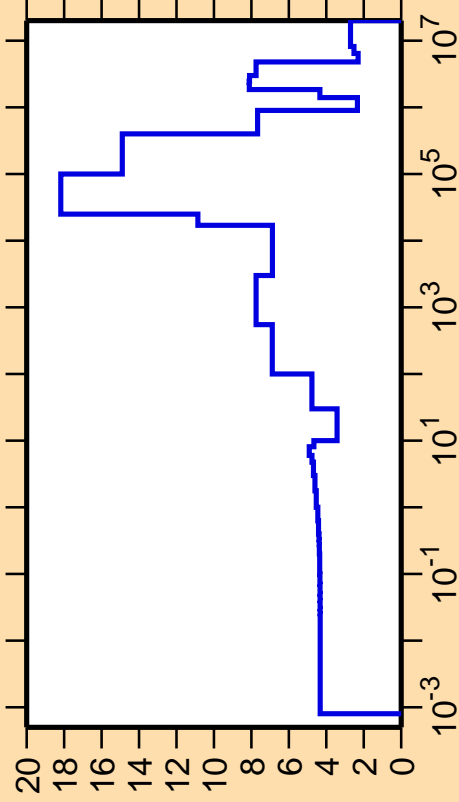
\Delta\sigma/\sigma vs. E for ^{121}\text{Te}(n,\text{el.})
