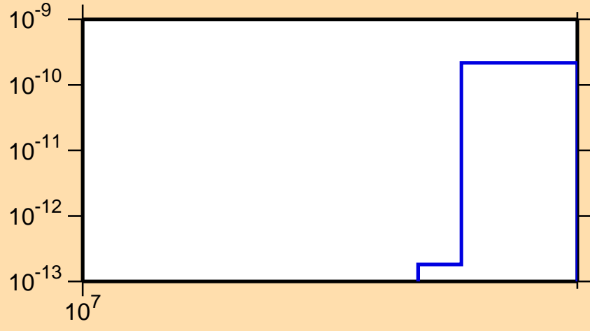
\sigma vs. E for ^{121}\text{Te}(n,\text{pt})
