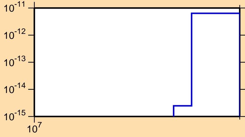
\sigma vs. E for ^{121}\text{Te} (mt 34)
