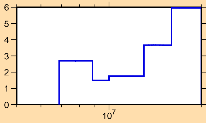
\Delta\sigma/\sigma vs. E for ^{121}\text{Te}(n,\text{el.})
