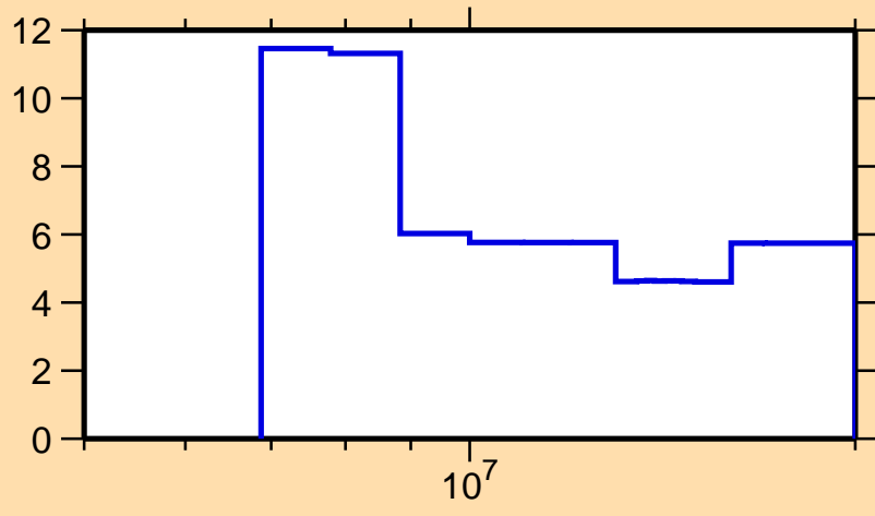
\Delta\sigma/\sigma vs. E for ^{121}\text{Te}(n,2n)
