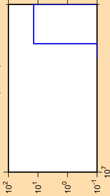
\Delta\sigma/\sigma vs. E for ^{121}\text{Te} (mt 34)
