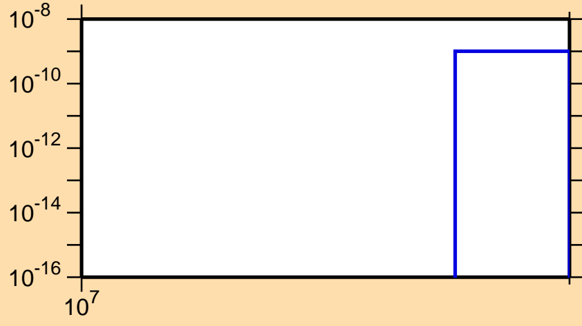
\sigma vs. E for ^{121}\text{Te}(n,nt)
