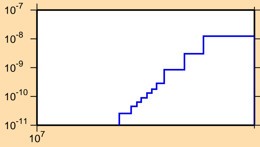
\sigma vs. E for ^{121}\text{Te}(n,p\alpha)
