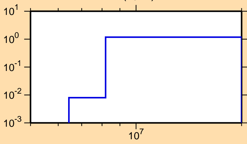
\sigma vs. E for ^{121}\text{Te}(n,2n)
