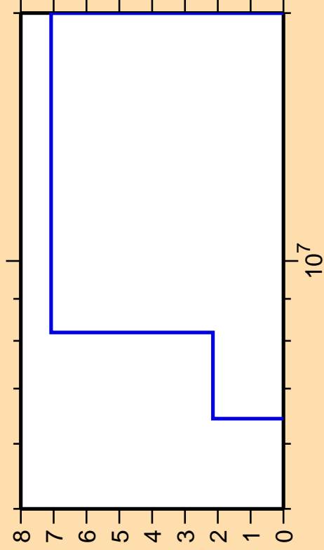
\Delta\sigma/\sigma vs. E for ^{121}\text{Te}(n,n\text{cont.})
