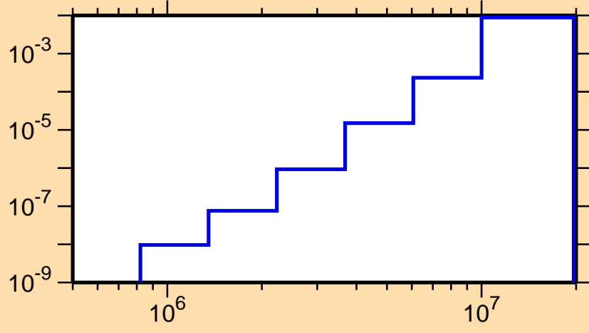
\sigma vs. E for ^{122}\text{Te}(n,\alpha)
