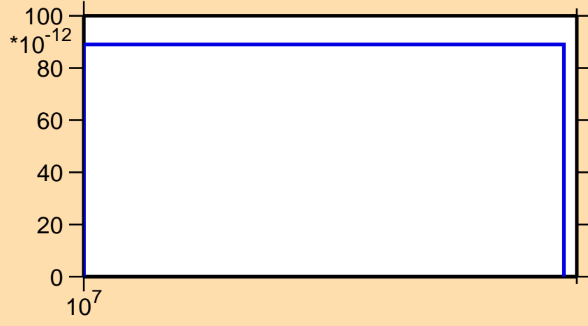
\sigma vs. E for ^{122}\text{Te}(n,nd)
