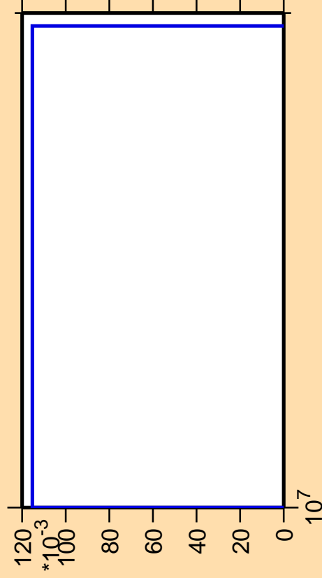
\Delta\sigma/\sigma vs. E for ^{122}\text{Te}(n,pd)
