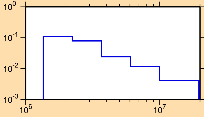
\sigma vs. E for ^{122}\text{Te}(n,n_4)
