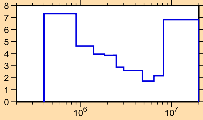
\Delta\sigma/\sigma vs. E for ^{122}\text{Te}(n,\text{inel.})
