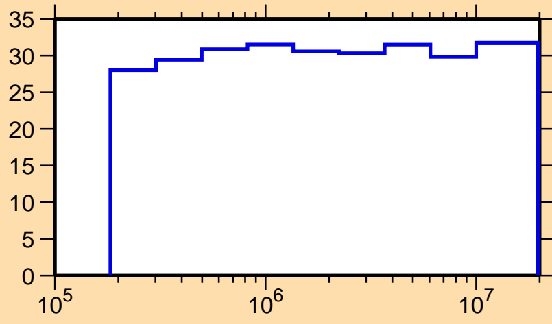
\Delta\sigma/\sigma vs. E for ^{123}\text{Te}(n,\gamma)
