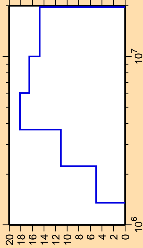
\Delta\sigma/\sigma vs. E for ^{124}\text{Te}(n,n_4)
