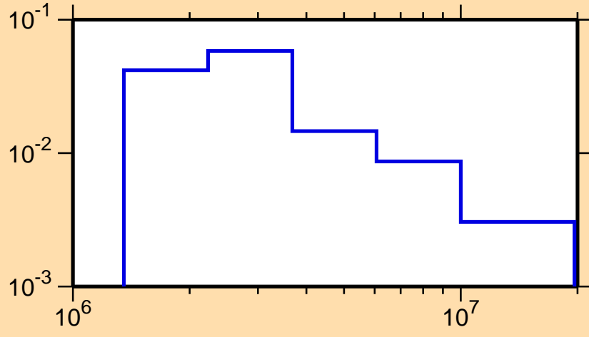
\sigma vs. E for ^{124}\text{Te}(n,n_4)
