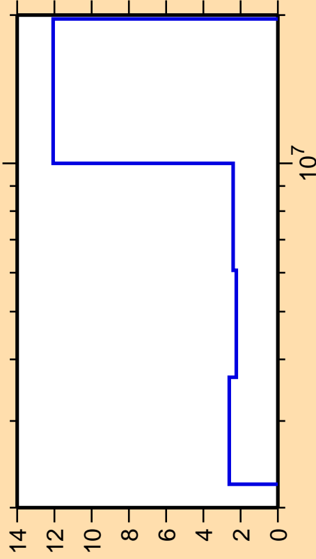
\Delta\sigma/\sigma vs. E for ^{124}\text{Te}(n,n\text{cont.})
