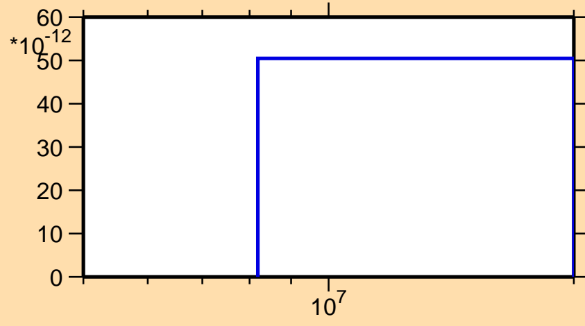
\sigma vs. E for ^{124}\text{Te}(n,nd)
