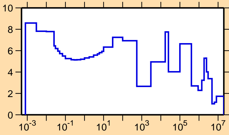
\Delta\sigma/\sigma vs. E for ^{124}\text{Te}(n,\text{tot.})
