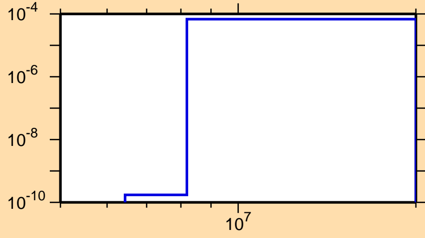
\sigma vs. E for ^{124}\text{Te}(n,n\alpha)
