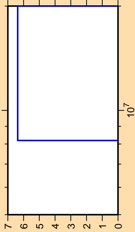
\Delta\sigma/\sigma vs. E for ^{124}\text{Te}(n,2n\alpha)
