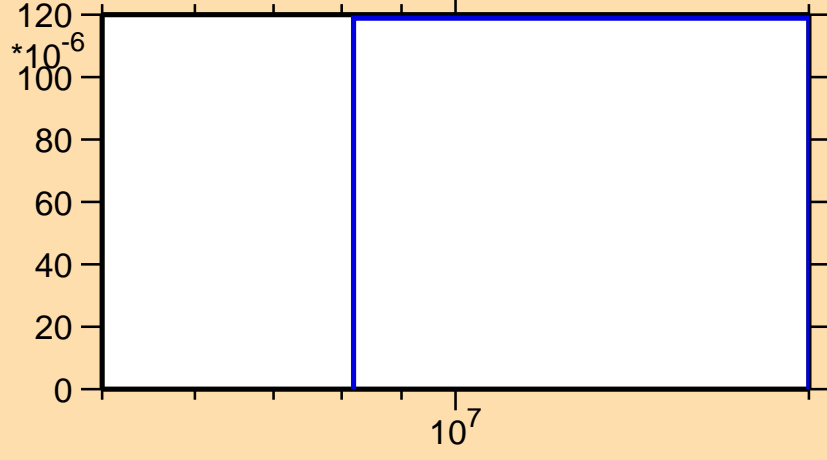
\sigma vs. E for ^{124}\text{Te}(n,3n)
