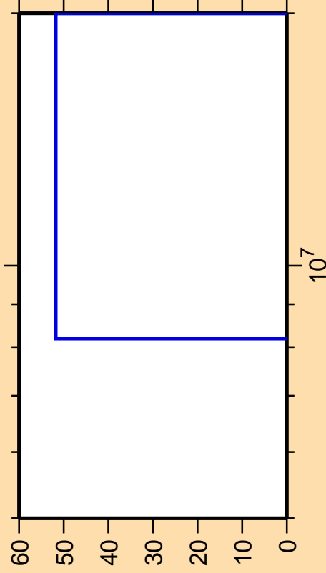
\Delta\sigma/\sigma vs. E for ^{124}\text{Te}(n,nd)
