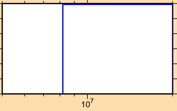
\sigma vs. E for ^{124}\text{Te}(n,3n)
