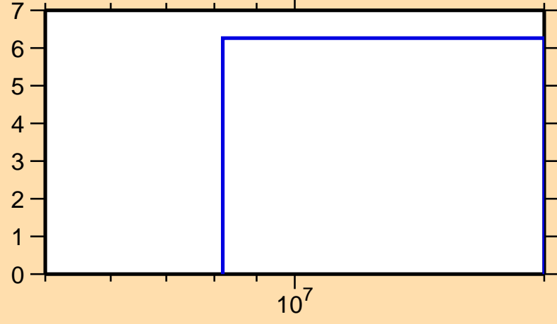
\Delta\sigma/\sigma vs. E for ^{124}\text{Te}(n,\text{inel.})
