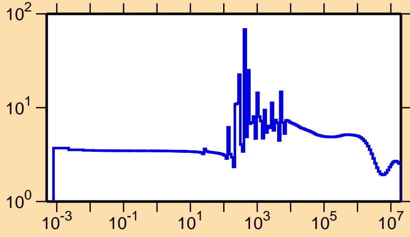
\sigma vs. E for ^{125}\text{Te}(n,\text{el.})
