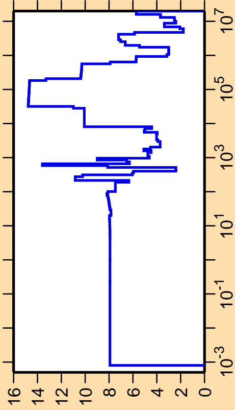
\Delta\sigma/\sigma vs. E for ^{125}\text{Te}(n,\text{el.})
