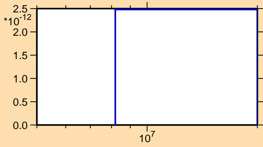
\sigma vs. E for ^{125}\text{Te}(n,nt)
