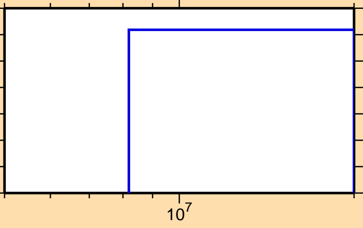
\sigma vs. E for ^{125}\text{Te}(n,d)
