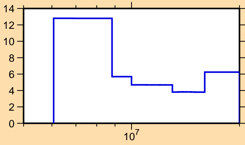
\Delta\sigma/\sigma vs. E for ^{125}\text{Te}(n,2n)
