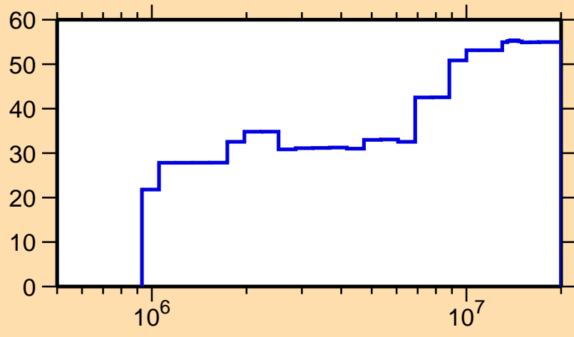
\Delta\sigma/\sigma vs. E for ^{125}\text{Te}(n,\gamma)
