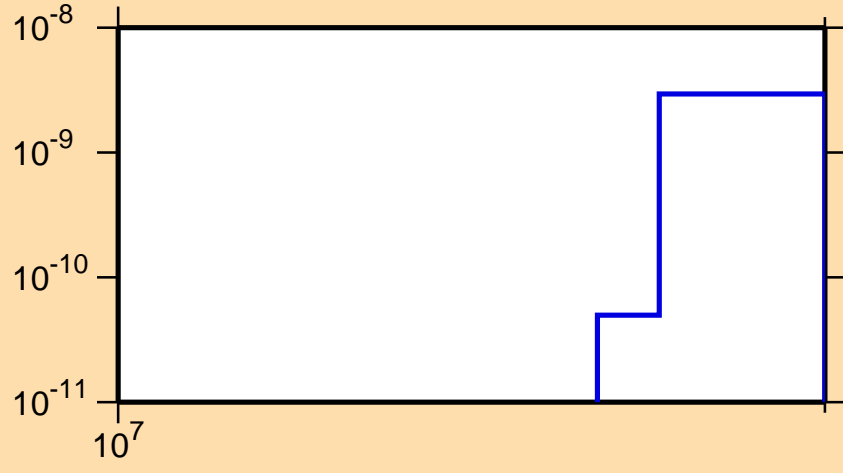
\sigma vs. E for ^{125}\text{Te}(n,\text{He3})
