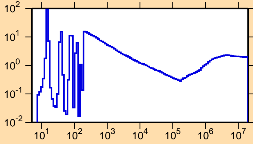
\sigma vs. E for ^{125}\text{Te}(n,\text{nonel.})
