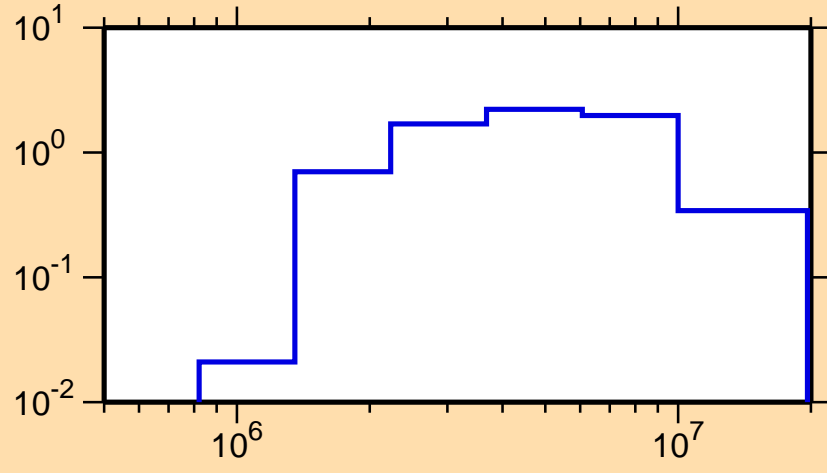
\sigma vs. E for ^{125}\text{Te}(n,n\text{cont.})
