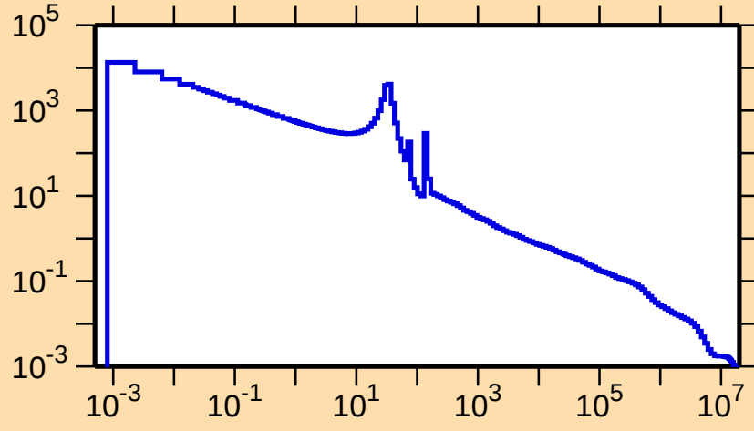
\sigma vs. E for ^{127}\text{Te}(n,\gamma)
