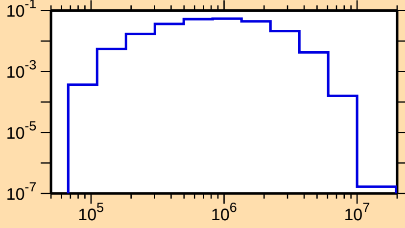
\sigma vs. E for ^{127}\text{Te}(n,n_2)
