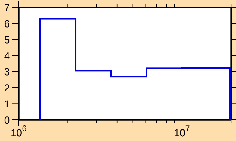
\Delta\sigma/\sigma vs. E for ^{127}\text{Te}(\text{n},\text{nonel.})
