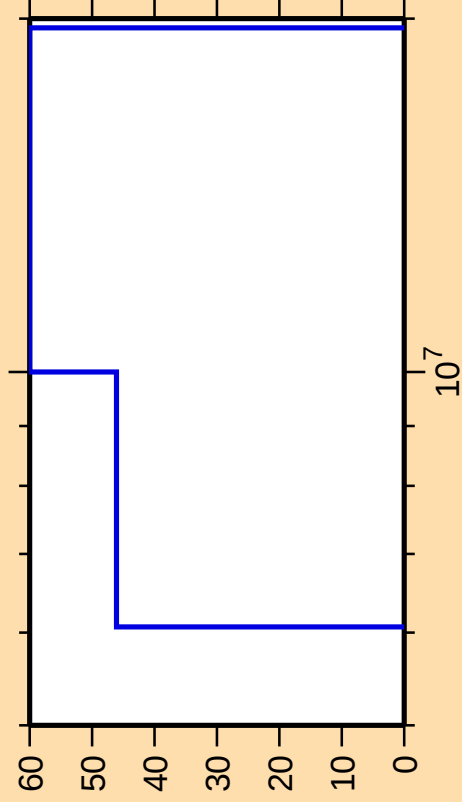
\Delta\sigma/\sigma vs. E for ^{127}\text{Te}(n,n_1)
