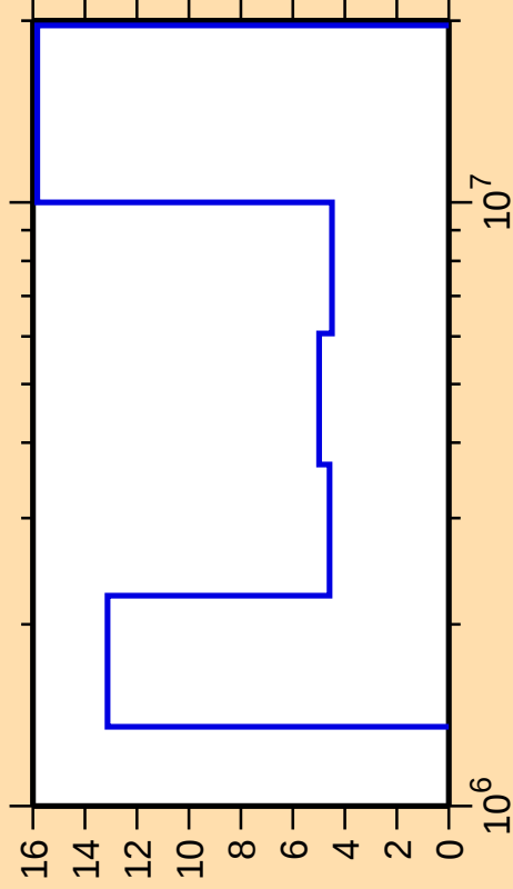
\Delta\sigma/\sigma vs. E for ^{127}\text{Te}(\text{n},\text{ncont.})
