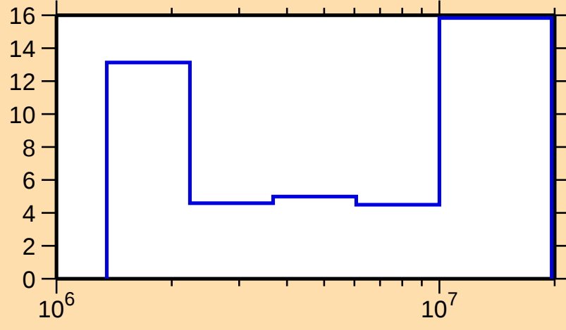
\Delta\sigma/\sigma vs. E for ^{127}\text{Te}(n,n\text{cont.})
