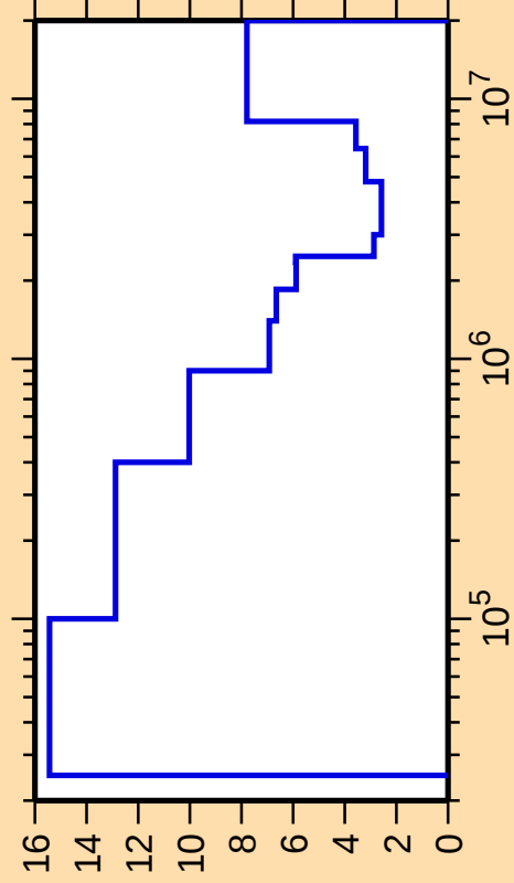
\Delta\sigma/\sigma vs. E for ^{127}\text{Te}(n,\text{inel.})
