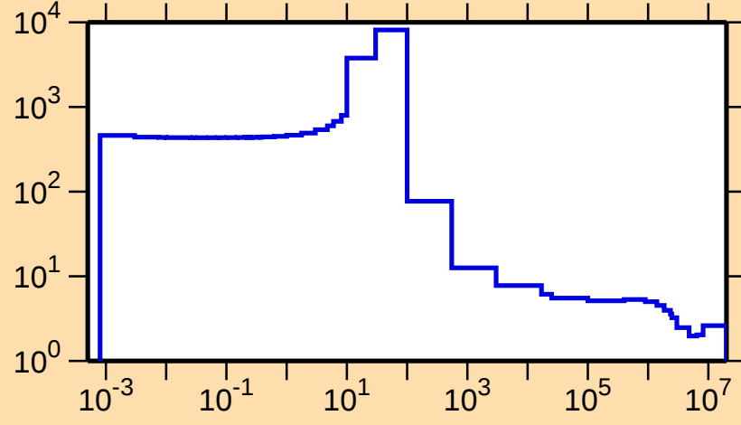
\sigma vs. E for ^{127}\text{Te}(n,\text{el.})
