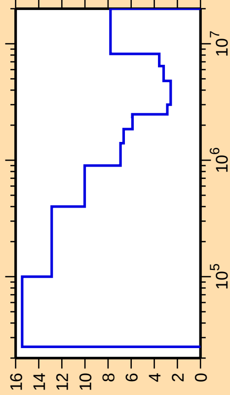
\Delta\sigma/\sigma vs. E for ^{127}\text{Te}(n,\text{inel.})
