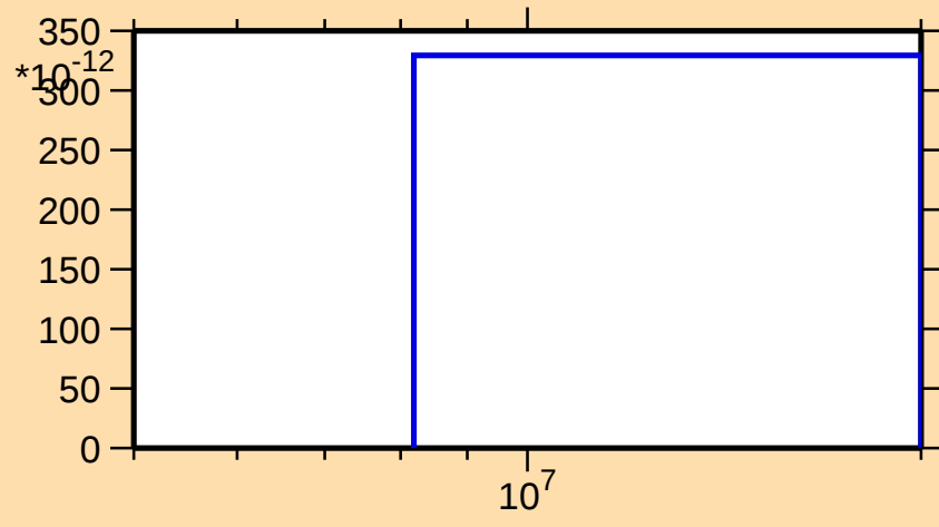
\sigma vs. E for ^{127}\text{Te}(n,2np)
