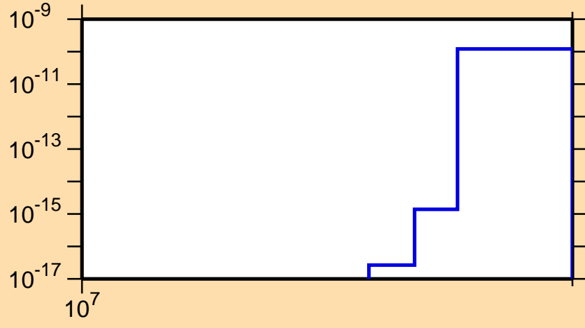
\sigma vs. E for ^{128}\text{Te}(n,nt)
