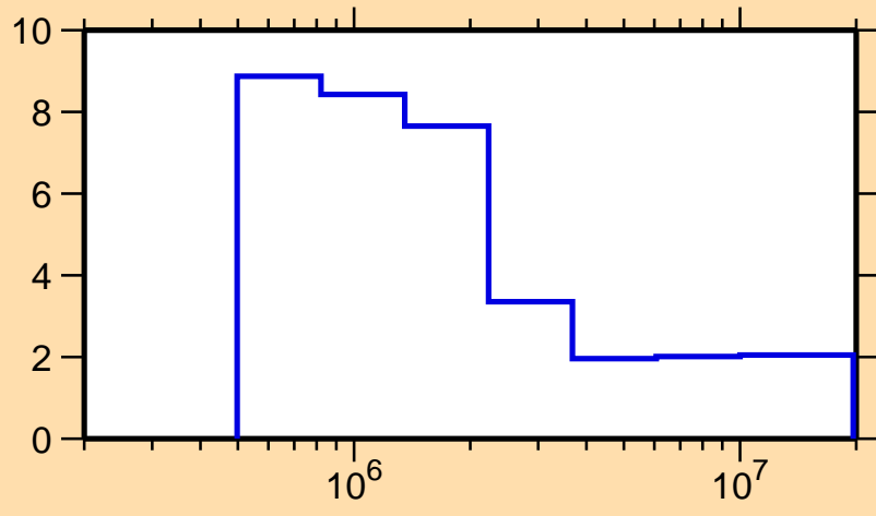
\Delta\sigma/\sigma vs. E for ^{128}\text{Te}(n,\text{nonel.})
