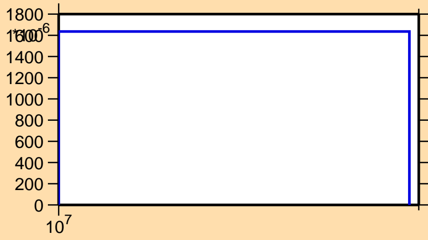
\sigma vs. E for ^{128}\text{Te}(n,3n)
