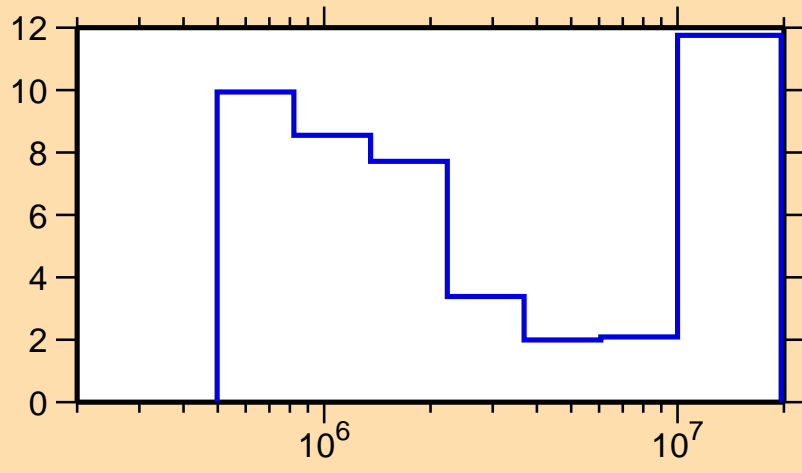
\Delta\sigma/\sigma vs. E for ^{128}\text{Te}(n,\text{inel.})
