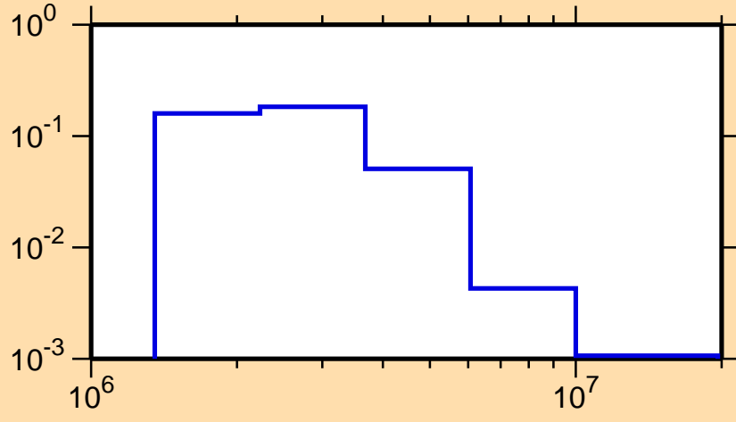
\sigma vs. E for ^{128}\text{Te}(n,n_3)
