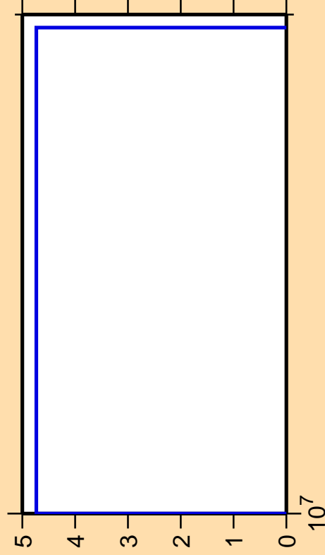
\Delta\sigma/\sigma vs. E for ^{128}\text{Te}(n,\text{nd})
