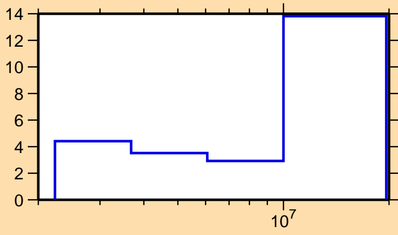
\Delta\sigma/\sigma vs. E for ^{128}\text{Te}(n,n\text{cont.})
