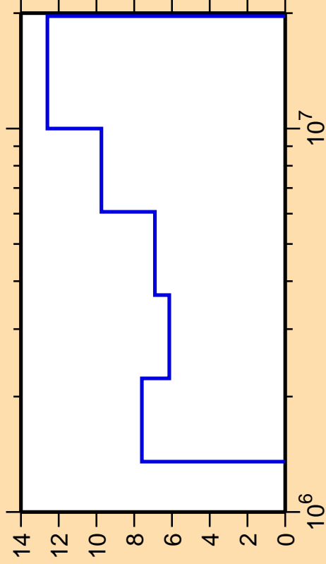
\Delta\sigma/\sigma vs. E for ^{128}\text{Te}(n,n_3)
