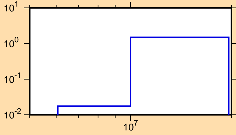
\sigma vs. E for ^{128}\text{Te}(n,2n)
