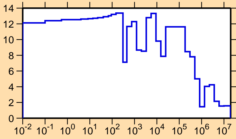
\Delta\sigma/\sigma vs. E for ^{128}\text{Te}(n,\text{tot.})
