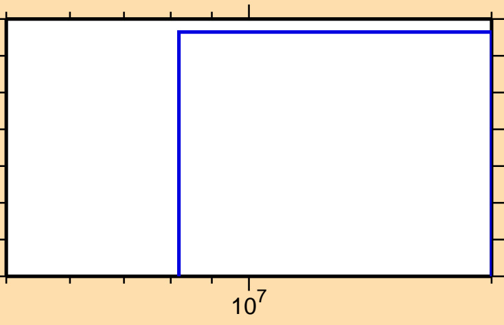
\sigma vs. E for ^{128}\text{Te}(n,3n)
