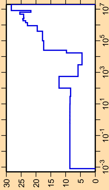
\Delta\sigma/\sigma vs. E for ^{128}\text{Te}(n,\gamma)
