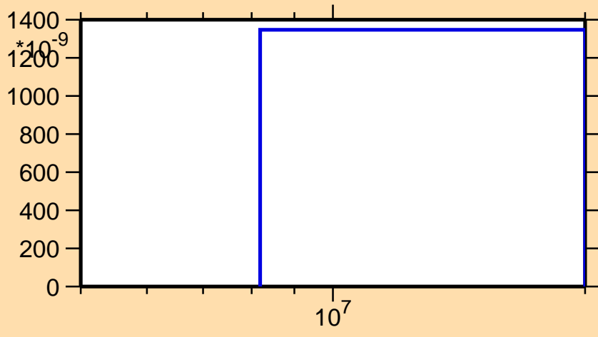
\sigma vs. E for ^{128}\text{Te}(n,t)
