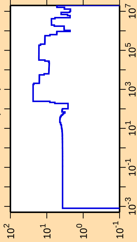
\Delta\sigma/\sigma vs. E for ^{129}\text{Te}(n,\text{el.})
