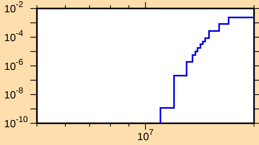
\sigma vs. E for ^{129}\text{Te}(n,np)
