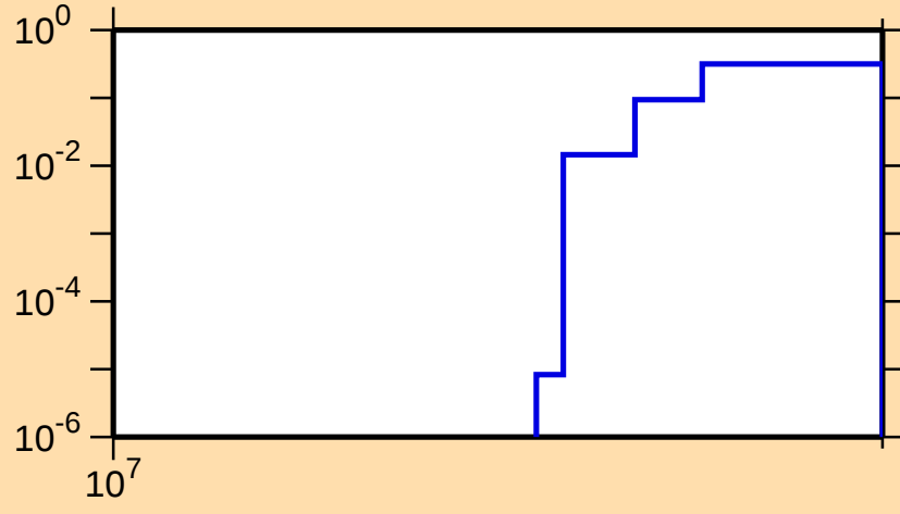
\sigma vs. E for ^{129}\text{Te}(n,3n)
