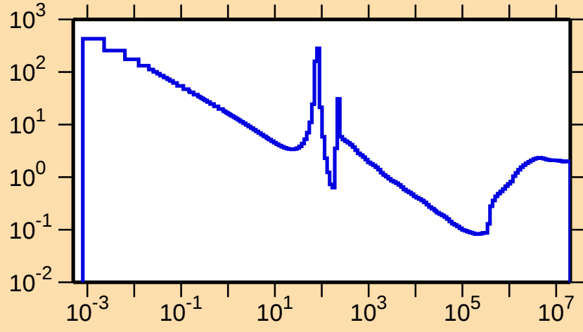
\sigma vs. E for ^{129}\text{Te}(n,\text{nonel.})
