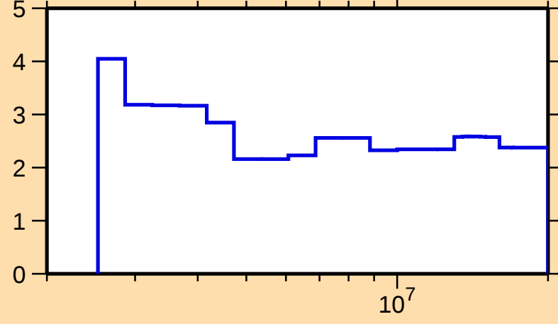
\Delta\sigma/\sigma vs. E for ^{129}\text{Te}(n,\text{nonel.})
