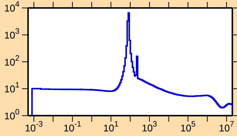
\sigma vs. E for ^{129}\text{Te}(n,\text{el.})
