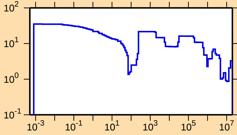
\Delta\sigma/\sigma vs. E for ^{129}\text{Te}(\text{n,tot.})
