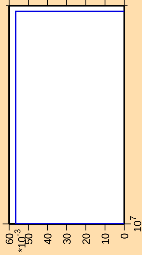
\Delta\sigma/\sigma vs. E for ^{129}\text{Te}(n,\text{He}3)
