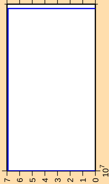
\Delta\sigma/\sigma vs. E for ^{129}\text{Te}(n,nt)
