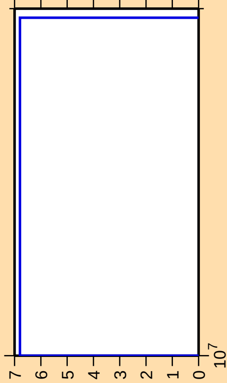
\Delta\sigma/\sigma vs. E for ^{129}\text{Te}(n,2n\alpha)
