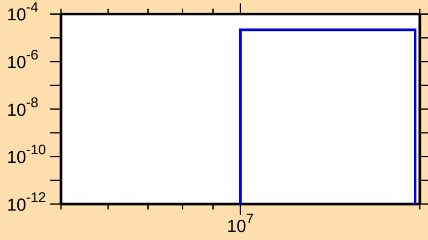
\sigma vs. E for ^{129}\text{Te}(n,t)
