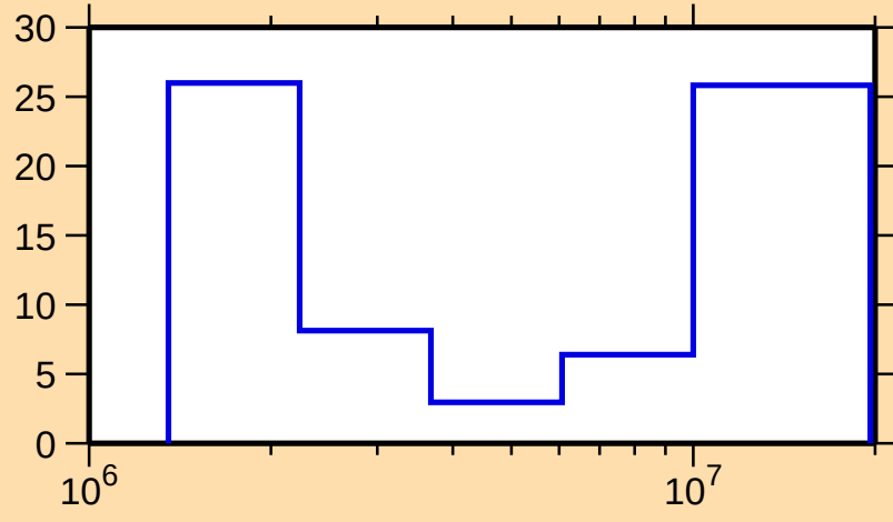
\Delta\sigma/\sigma vs. E for ^{129}\text{Te}(n,n\text{cont.})
