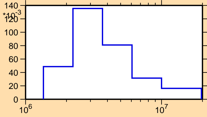
\sigma vs. E for ^{130}\text{Te}(n,n_3)
