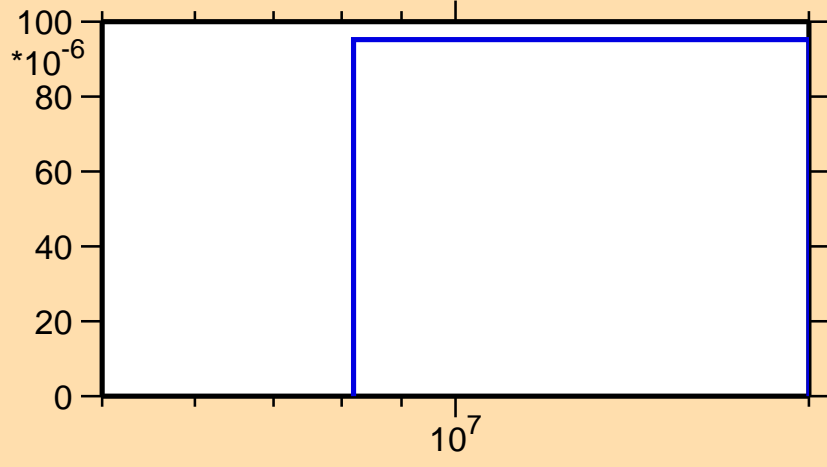
\sigma vs. E for ^{130}\text{Te}(n,d)
