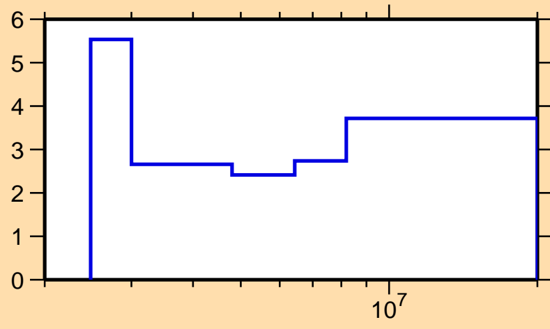
\Delta\sigma/\sigma vs. E for ^{130}\text{Te}(n,\text{inel.})
