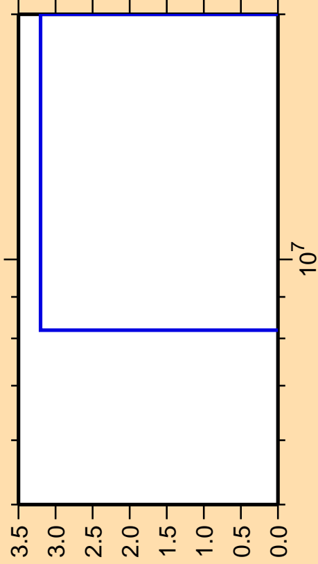
\Delta\sigma/\sigma vs. E for ^{130}\text{Te}(n,nd)
