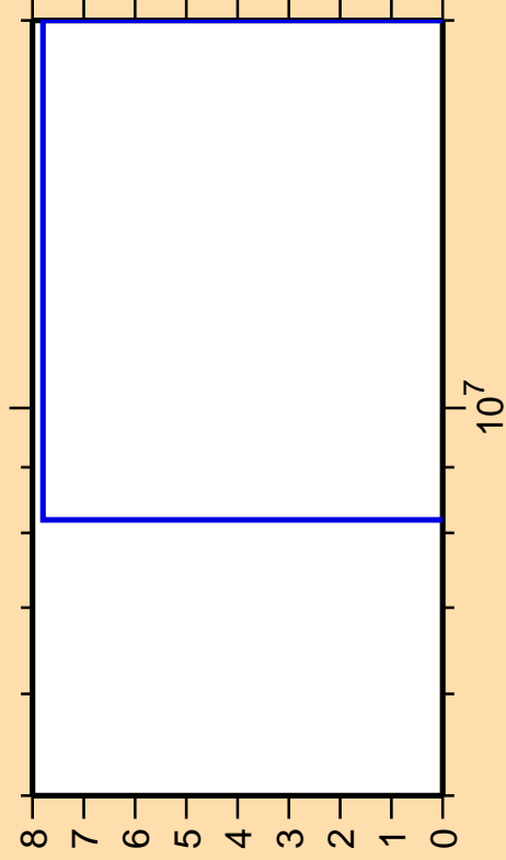
\Delta\sigma/\sigma vs. E for ^{130}\text{Te}(n,3n)
