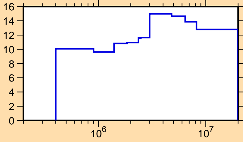
\Delta\sigma/\sigma vs. E for ^{130}\text{Te}(n,n_1)
