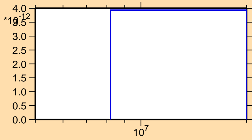
\sigma vs. E for ^{130}\text{Te}(n,nd)
