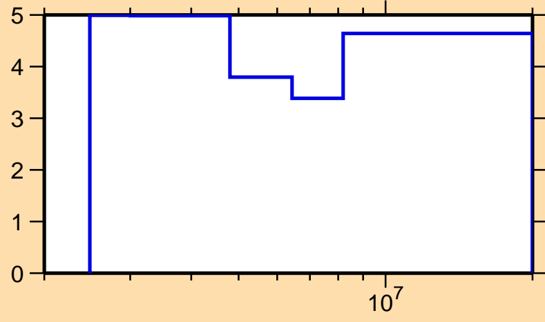
\Delta\sigma/\sigma vs. E for ^{130}\text{Te}(n,n\text{cont.})
