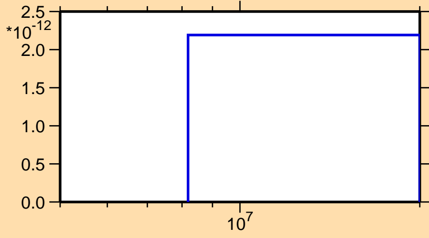
\sigma vs. E for ^{130}\text{Te}(n,nt)
