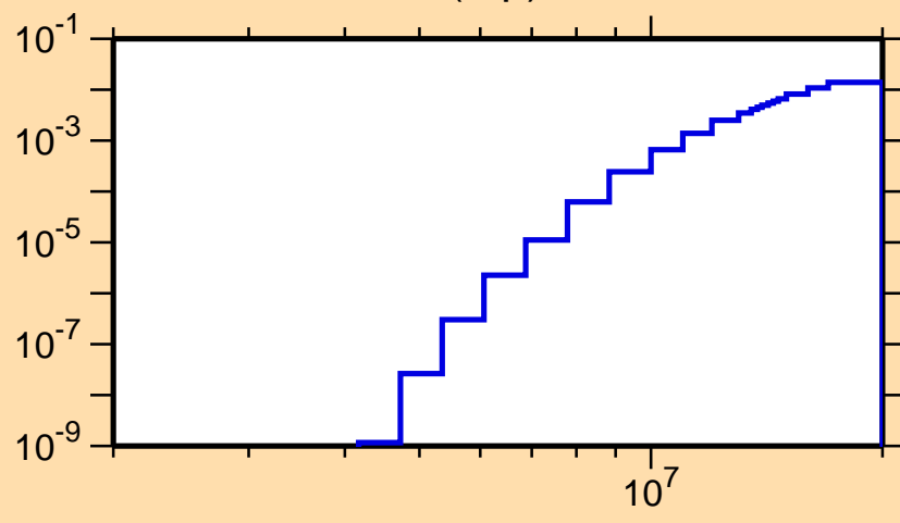
\sigma vs. E for ^{131}\text{Te}(n,p)
