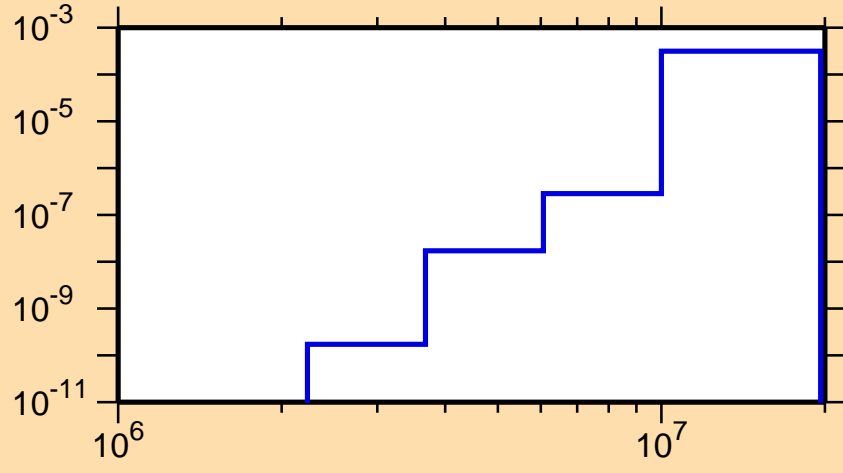
\sigma vs. E for ^{131}\text{Te}(n,\alpha)
