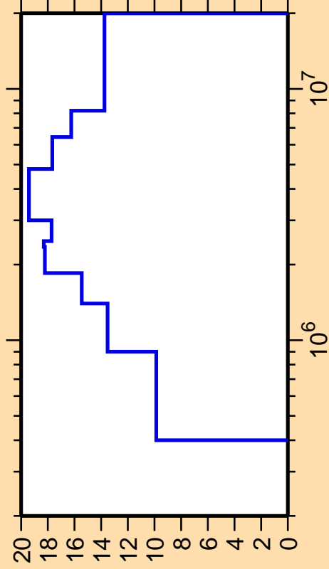
\Delta\sigma/\sigma vs. E for ^{131}\text{Te}(n,n_3)
