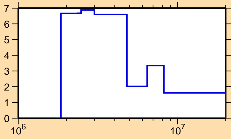
\Delta\sigma/\sigma vs. E for ^{131}\text{Te}(n,\text{el.})
