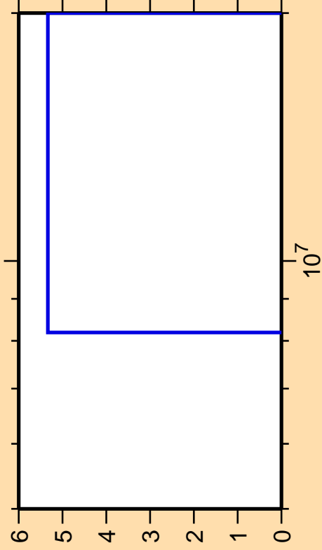
\Delta\sigma/\sigma vs. E for ^{131}\text{Te}(n,nt)
