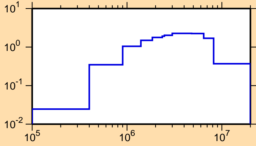
\sigma vs. E for ^{131}\text{Te}(n,\text{inel.})
