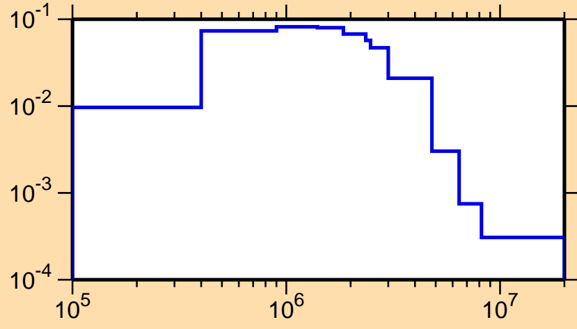
\sigma vs. E for ^{131}\text{Te}(n,n_1)
