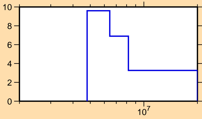
\Delta\sigma/\sigma vs. E for ^{131}\text{Te}(n,2n)
