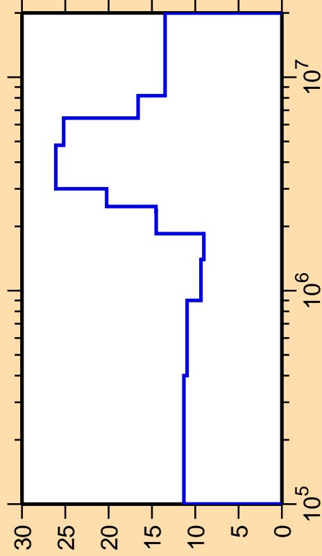
\Delta\sigma/\sigma vs. E for ^{131}\text{Te}(n,n_1)
