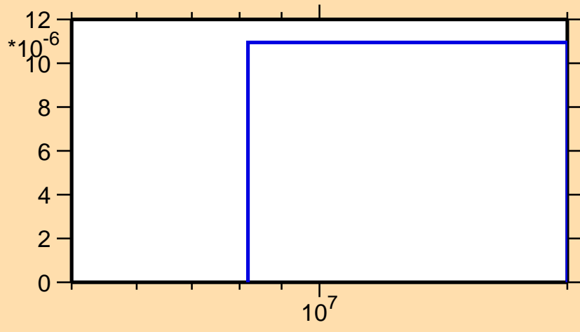
\sigma vs. E for ^{131}\text{Te}(n,t)
