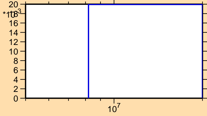
\sigma vs. E for ^{131}\text{Te}(n,3n)
