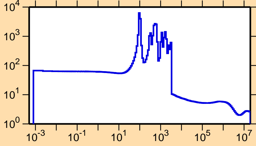
\sigma vs. E for ^{131}\text{Te}(n,\text{el.})
