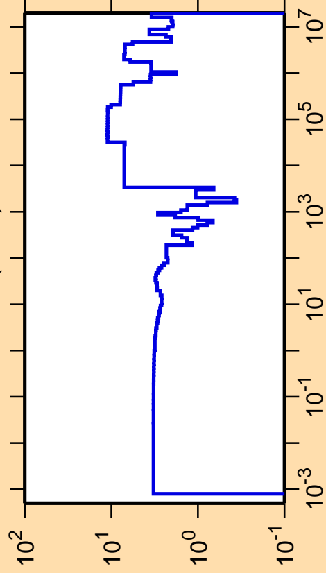
\Delta\sigma/\sigma vs. E for ^{131}\text{Te}(n,\text{el.})
