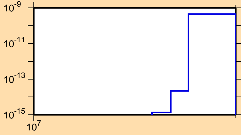
\sigma vs. E for ^{132}\text{Te}(n,nt)
