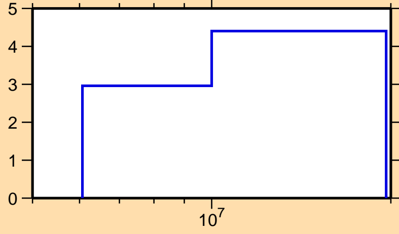
\Delta\sigma/\sigma vs. E for ^{132}\text{Te}(n,\text{el.})
