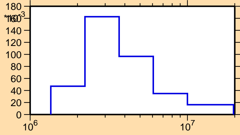
\sigma vs. E for ^{132}\text{Te}(n,n_3)
