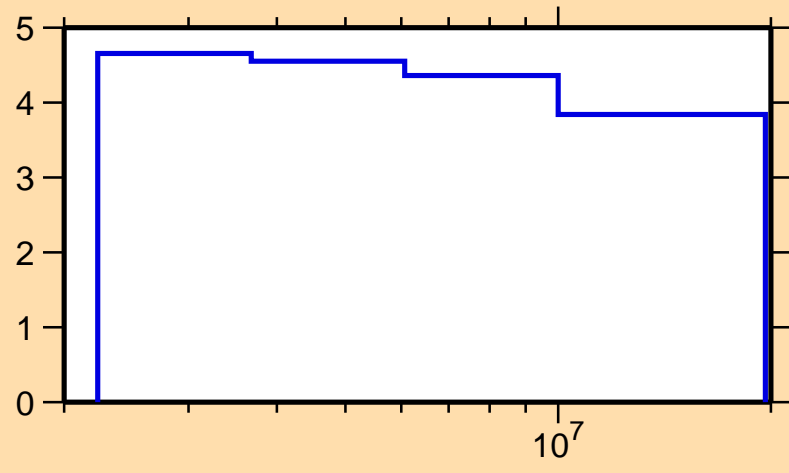
\Delta\sigma/\sigma vs. E for ^{132}\text{Te}(n,n\text{onel.})
