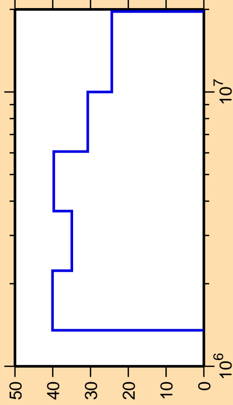
\Delta\sigma/\sigma vs. E for ^{132}\text{Te}(n,n_4)
