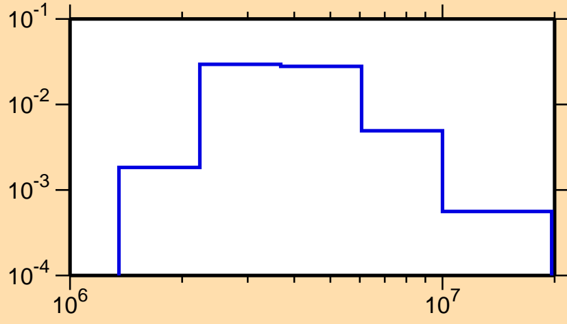
\sigma vs. E for ^{132}\text{Te}(n,n_4)
