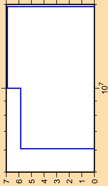
\Delta\sigma/\sigma vs. E for ^{132}\text{Te}(n,2n)
