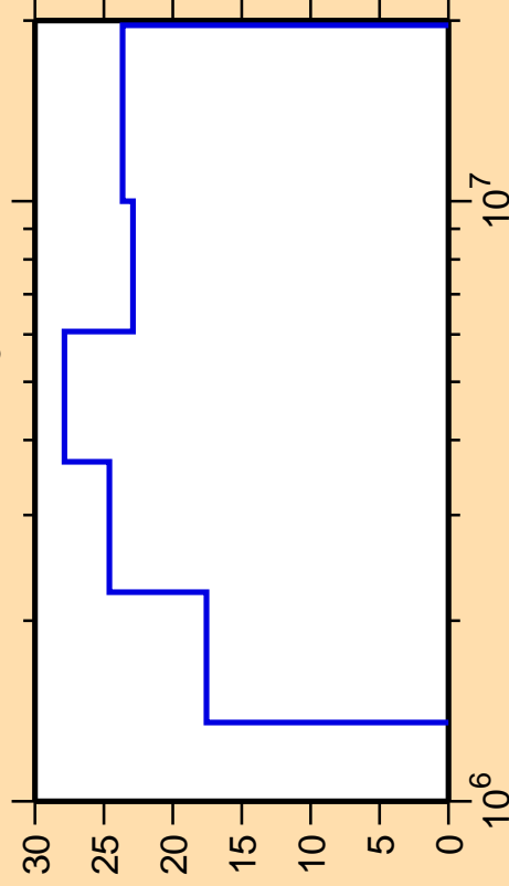
\Delta\sigma/\sigma vs. E for ^{132}\text{Te}(n,n_3)
