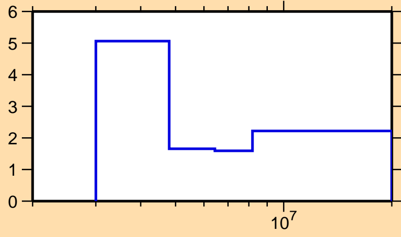
\Delta\sigma/\sigma vs. E for ^{132}\text{Te}(n,\text{tot.})
