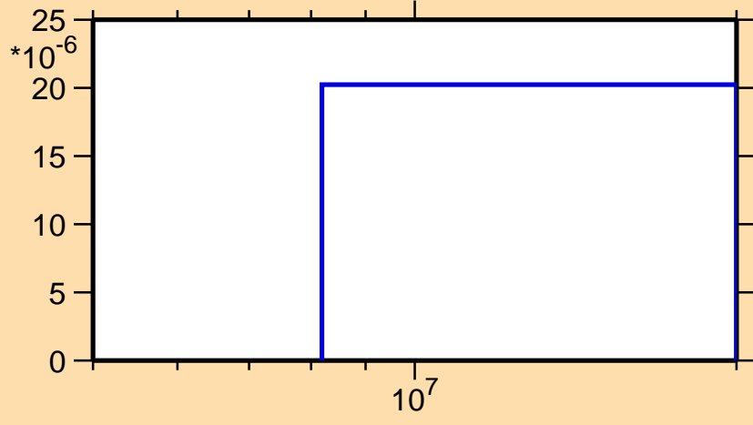
\sigma vs. E for ^{132}\text{Te}(n,np)
