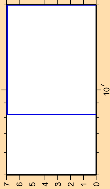
\Delta\sigma/\sigma vs. E for ^{132}\text{Te}(n,\text{nd})
