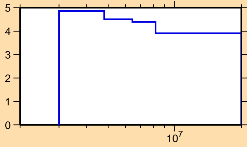
\Delta\sigma/\sigma vs. E for ^{132}\text{Te}(n,\text{nonel.})
