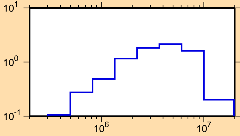
\sigma vs. E for ^{133}\text{Te}(n,\text{inel.})
