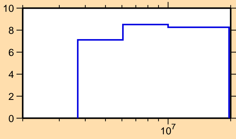
\Delta\sigma/\sigma vs. E for ^{133}\text{Te}(n,n\text{onel.})
