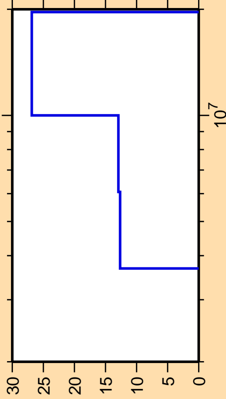
\Delta\sigma/\sigma vs. E for ^{133}\text{Te}(n,n\text{cont.})
