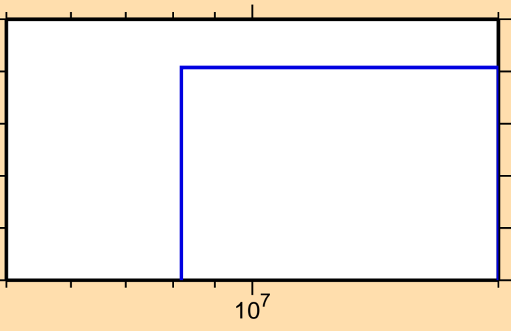
\sigma vs. E for ^{133}\text{Te}(n,2np)
