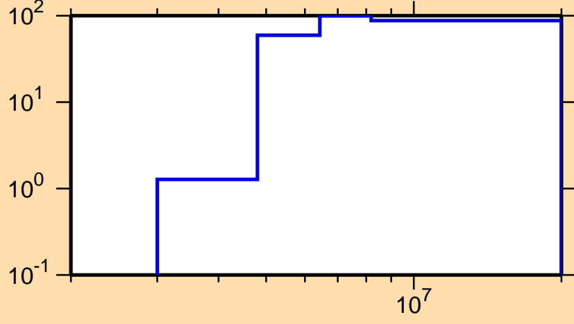
\Delta\sigma/\sigma vs. E for ^{133}\text{Te}(n,p)
