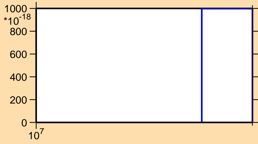
\sigma vs. E for ^{134}\text{Te}(n,2np)
