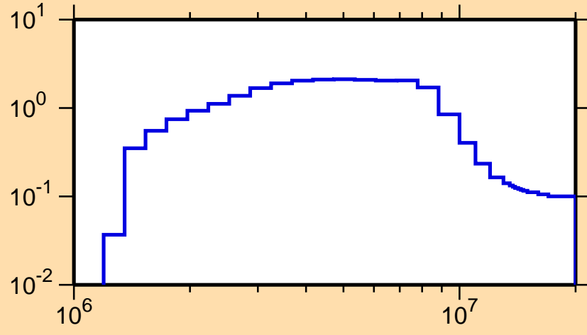
\sigma vs. E for ^{134}\text{Te}(n,\text{inel.})
