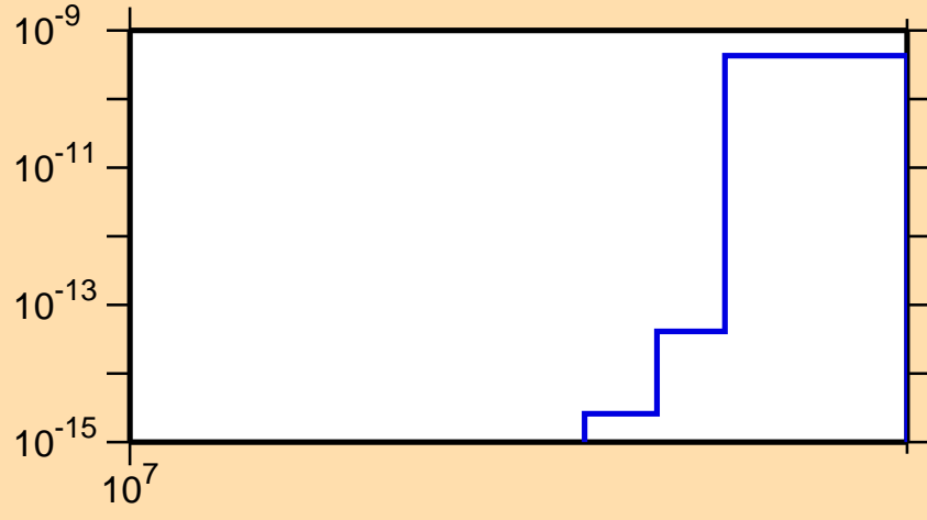
\sigma vs. E for ^{134}\text{Te}(n,nt)
