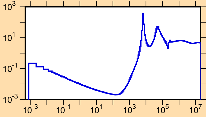
\sigma vs. E for ^{134}\text{Te}(n,\text{tot.})
