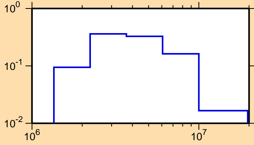
\sigma vs. E for ^{134}\text{Te}(n,n_2)
