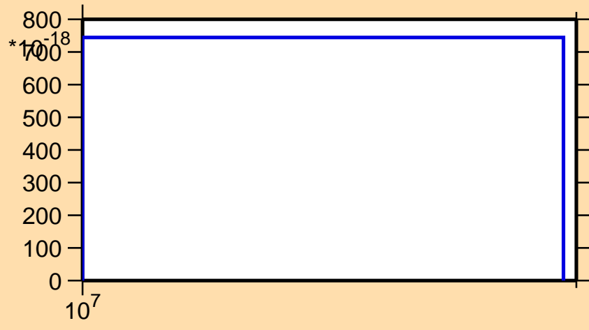
\sigma vs. E for ^{134}\text{Te}(n,2n\alpha)
