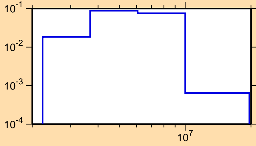
\sigma vs. E for ^{134}\text{Te}(n,n_4)
