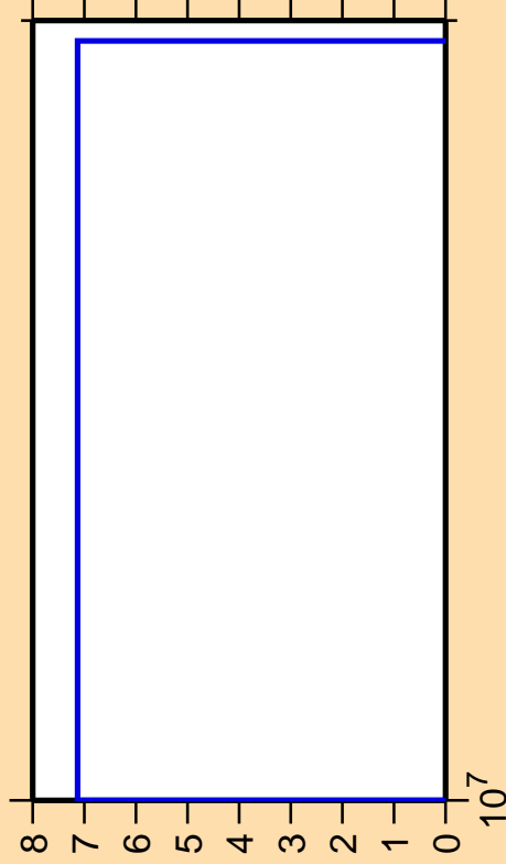
\Delta\sigma/\sigma vs. E for ^{134}\text{Te}(n,\text{nd})
