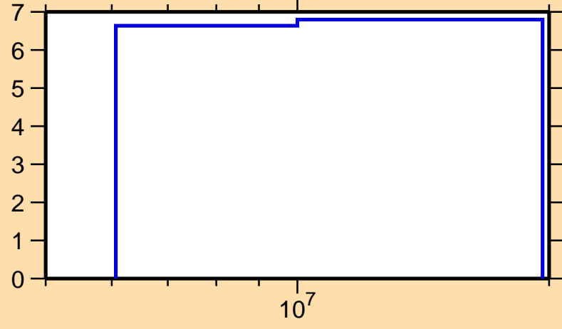
\Delta\sigma/\sigma vs. E for ^{134}\text{Te}(n,n\text{onl.})
