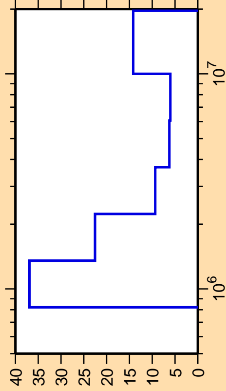
\Delta\sigma/\sigma vs. E for ^{134}\text{Te}(n,\text{inel.})
