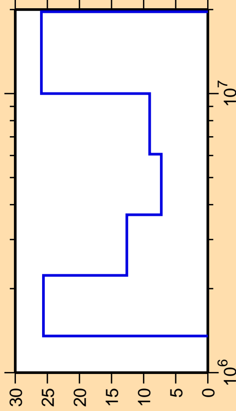
\Delta\sigma/\sigma vs. E for ^{134}\text{Te}(n,n_2)
